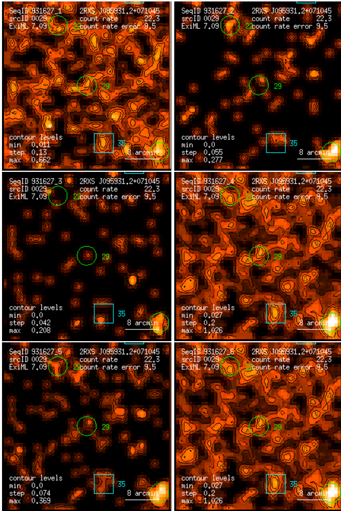
Figure 29: RASS 931627: detection 0029: band rate images, Gaussian filter: (1) PSPC channels 11 – 41, (2) 52 – 90, (3) 91 – 201, (4) 11 – 235, (5) 52 – 201, (6) 11 – 201. Broad band rates in counts/ks. Band rate contour levels in counts/ks/arcmin 2 .
