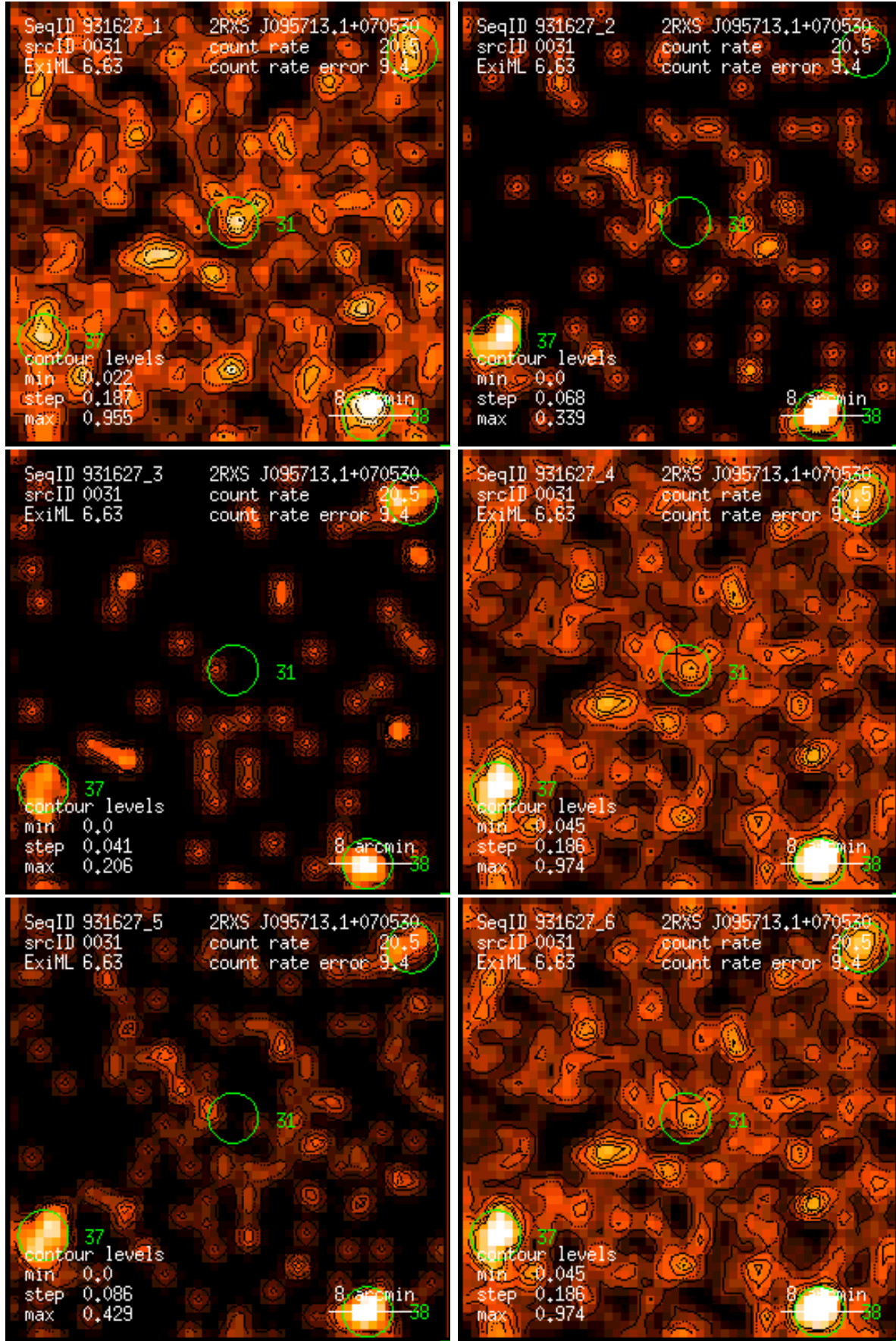
Figure 31: RASS 931627: detection 0031: band rate images, Gaussian filter: (1) PSPC channels 11 – 41, (2) 52 – 90, (3) 91 – 201, (4) 11 – 235, (5) 52 – 201, (6) 11 – 201. Broad band rates in counts/ks. Band rate contour levels in counts/ks/arcmin 2 .
