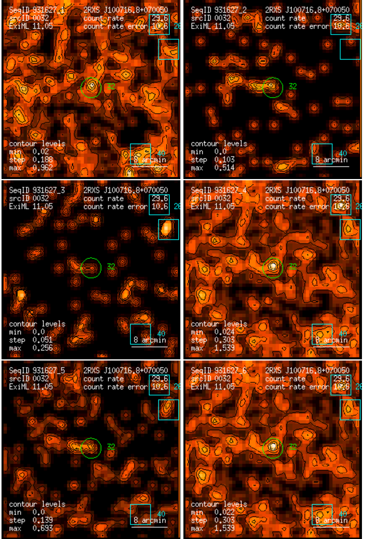
Figure 32: RASS 931627: detection 0032: band rate images, Gaussian filter: (1) PSPC channels 11 – 41, (2) 52 – 90, (3) 91 – 201, (4) 11 – 235, (5) 52 – 201, (6) 11 – 201. Broad band rates in counts/ks. Band rate contour levels in counts/ks/arcmin 2 .
