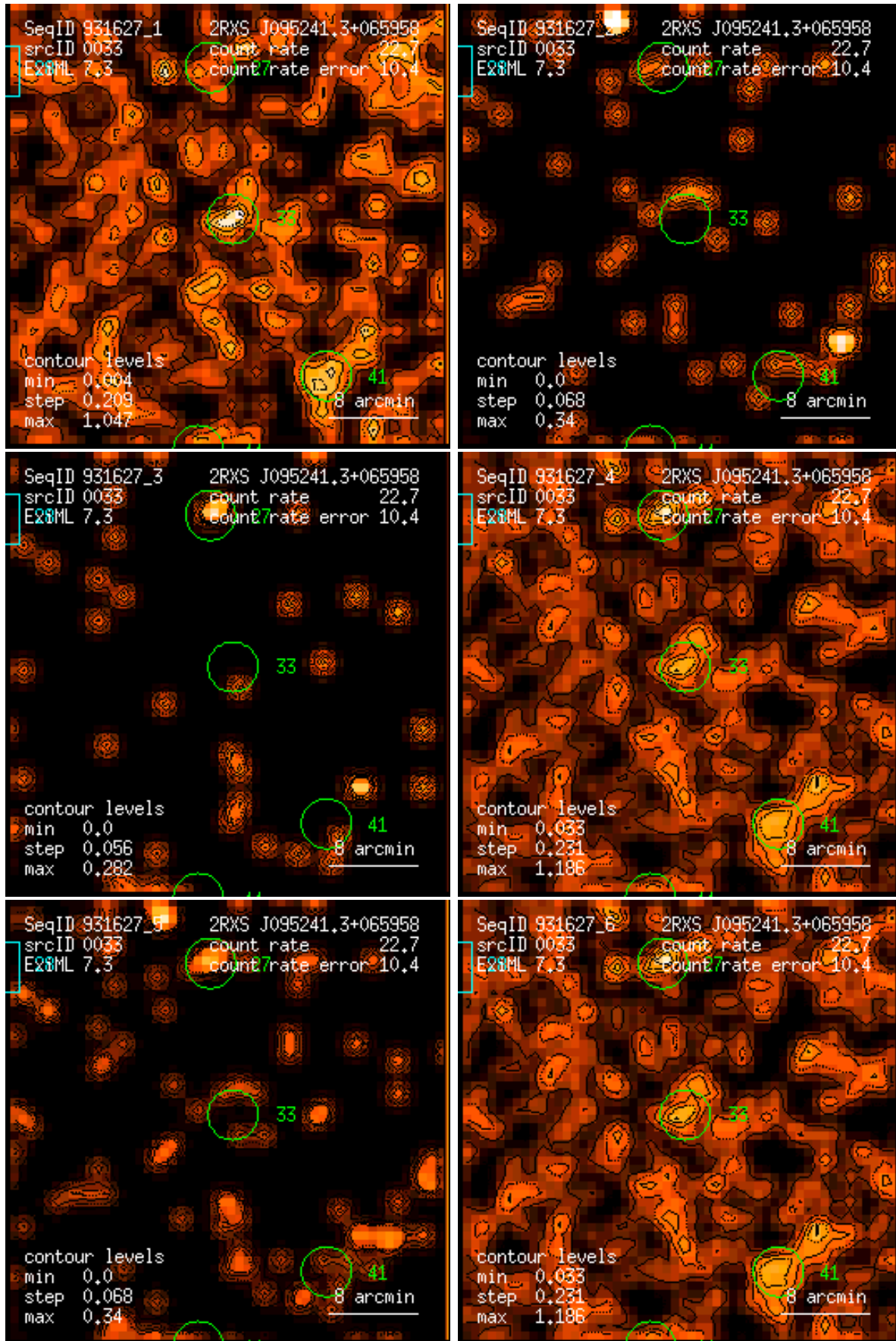
Figure 33: RASS 931627: detection 0033: band rate images, Gaussian filter: (1) PSPC channels 11 – 41, (2) 52 – 90, (3) 91 – 201, (4) 11 – 235, (5) 52 – 201, (6) 11 – 201. Broad band rates in counts/ks. Band rate contour levels in counts/ks/arcmin 2 .
