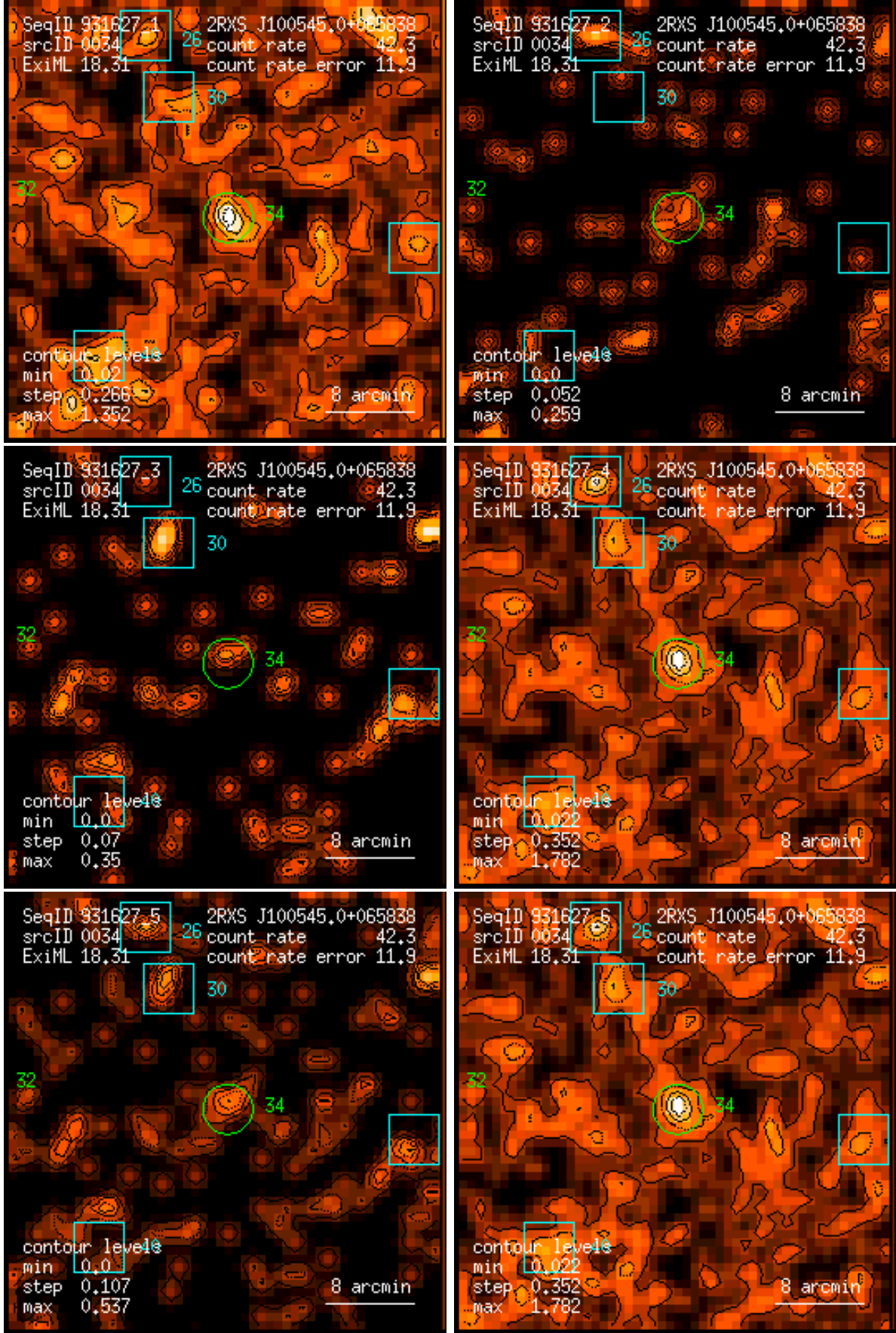
Figure 34: RASS 931627: detection 0034: band rate images, Gaussian filter: (1) PSPC channels 11 – 41, (2) 52 – 90, (3) 91 – 201, (4) 11 – 235, (5) 52 – 201, (6) 11 – 201. Broad band rates in counts/ks. Band rate contour levels in counts/ks/arcmin 2 .
