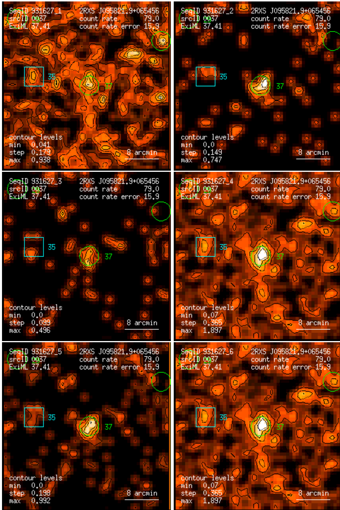
Figure 37: RASS 931627: detection 0037: band rate images, Gaussian filter: (1) PSPC channels 11 – 41, (2) 52 – 90, (3) 91 – 201, (4) 11 – 235, (5) 52 – 201, (6) 11 – 201. Broad band rates in counts/ks. Band rate contour levels in counts/ks/arcmin 2 .
