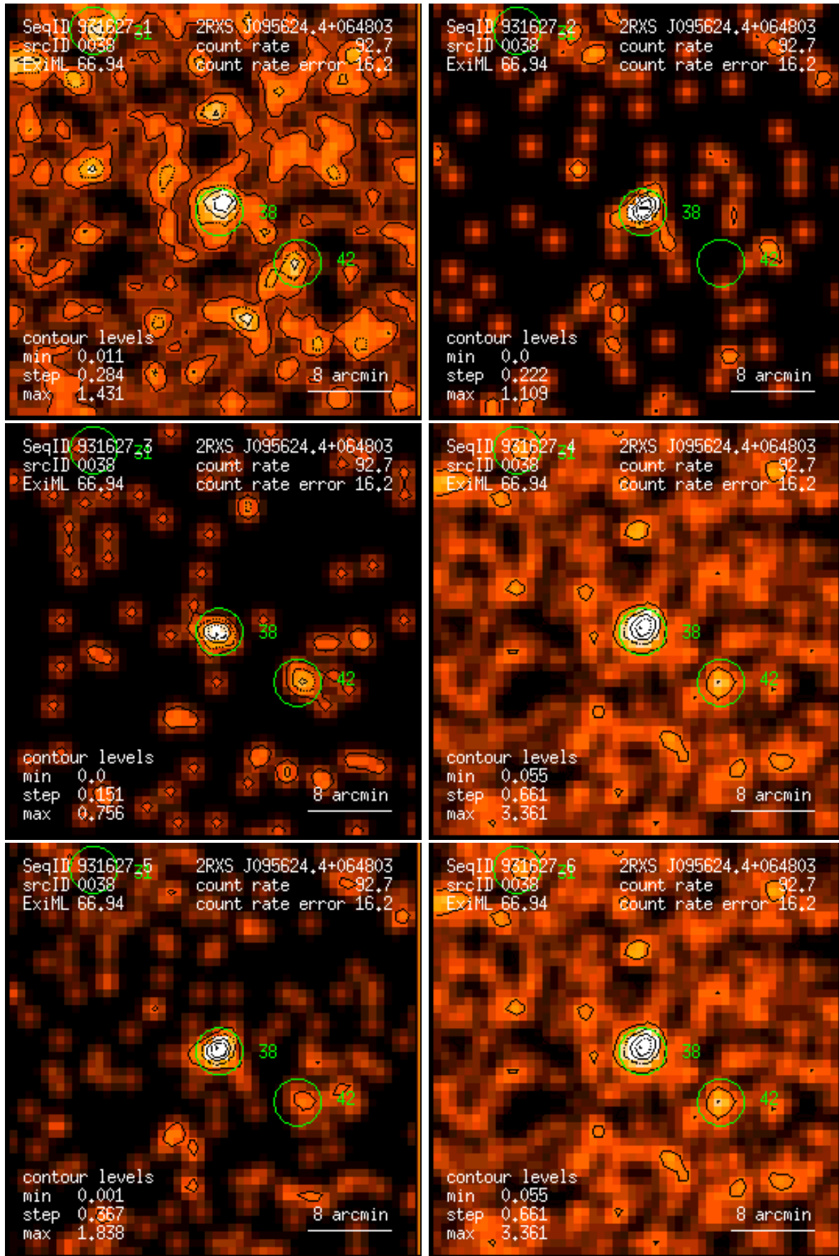
Figure 38: RASS 931627: detection 0038: band rate images, Gaussian filter: (1) PSPC channels 11 – 41, (2) 52 – 90, (3) 91 – 201, (4) 11 – 235, (5) 52 – 201, (6) 11 – 201. Broad band rates in counts/ks. Band rate contour levels in counts/ks/arcmin 2 .
