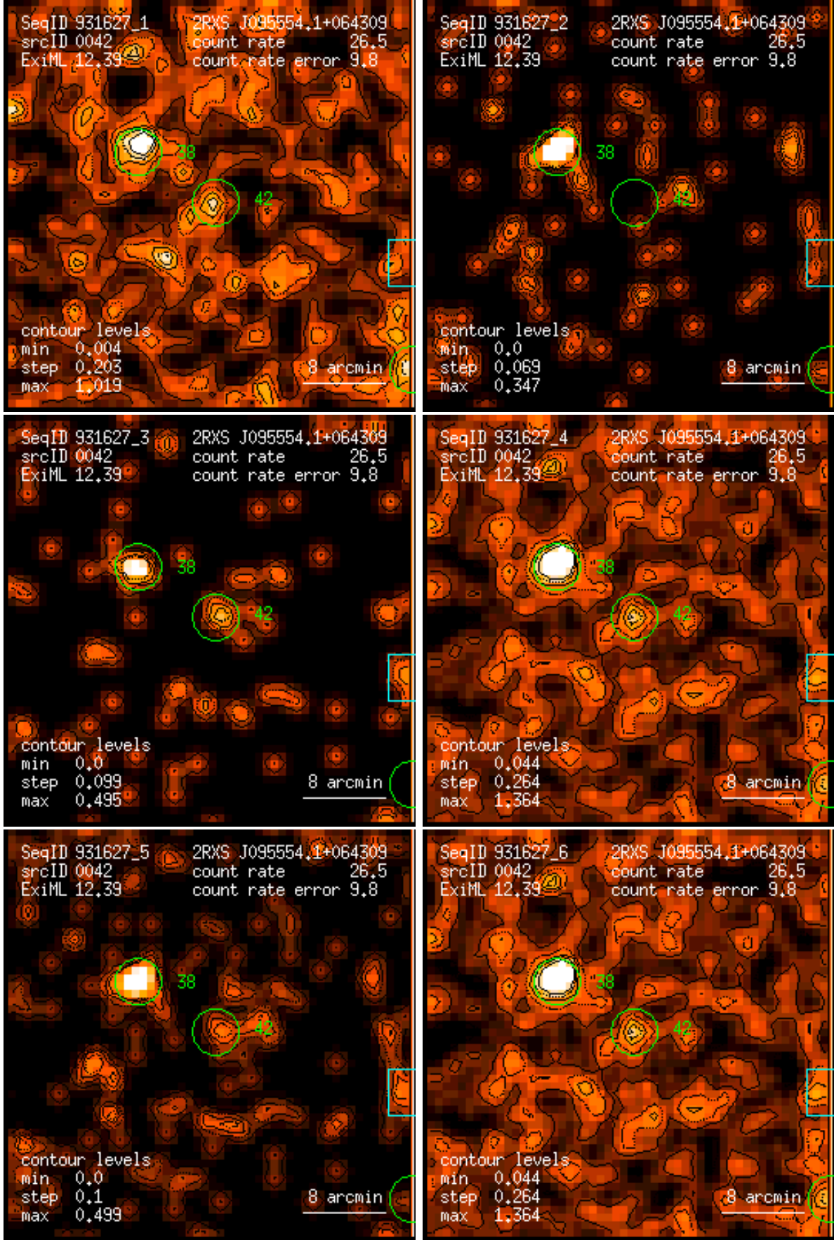
Figure 42: RASS 931627: detection 0042: band rate images, Gaussian filter: (1) PSPC channels 11 – 41, (2) 52 – 90, (3) 91 – 201, (4) 11 – 235, (5) 52 – 201, (6) 11 – 201. Broad band rates in counts/ks. Band rate contour levels in counts/ks/arcmin 2 .
