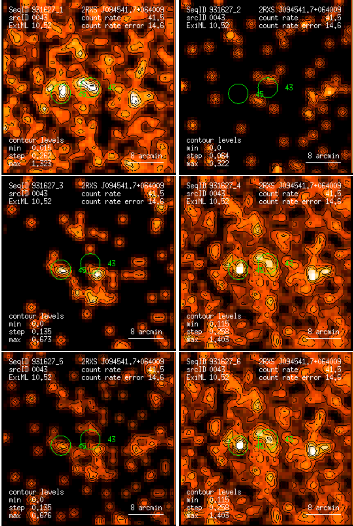
Figure 43: RASS 931627: detection 0043: band rate images, Gaussian filter: (1) PSPC channels 11 – 41, (2) 52 – 90, (3) 91 – 201, (4) 11 – 235, (5) 52 – 201, (6) 11 – 201. Broad band rates in counts/ks. Band rate contour levels in counts/ks/arcmin 2 .
