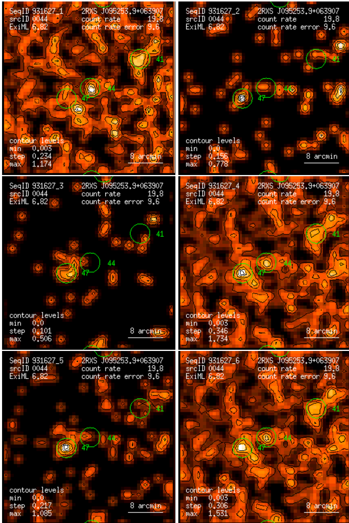
Figure 44: RASS 931627: detection 0044: band rate images, Gaussian filter: (1) PSPC channels 11 – 41, (2) 52 – 90, (3) 91 – 201, (4) 11 – 235, (5) 52 – 201, (6) 11 – 201. Broad band rates in counts/ks. Band rate contour levels in counts/ks/arcmin 2 .
