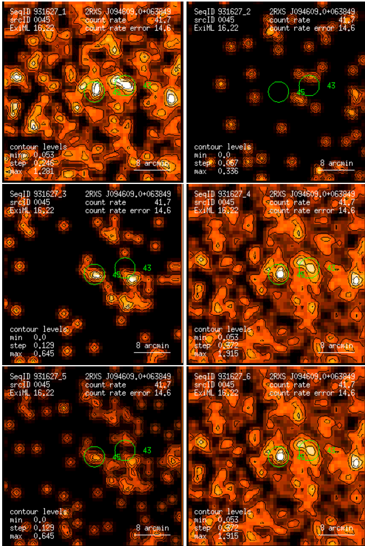
Figure 45: RASS 931627: detection 0045: band rate images, Gaussian filter: (1) PSPC channels 11 – 41, (2) 52 – 90, (3) 91 – 201, (4) 11 – 235, (5) 52 – 201, (6) 11 – 201. Broad band rates in counts/ks. Band rate contour levels in counts/ks/arcmin 2 .
