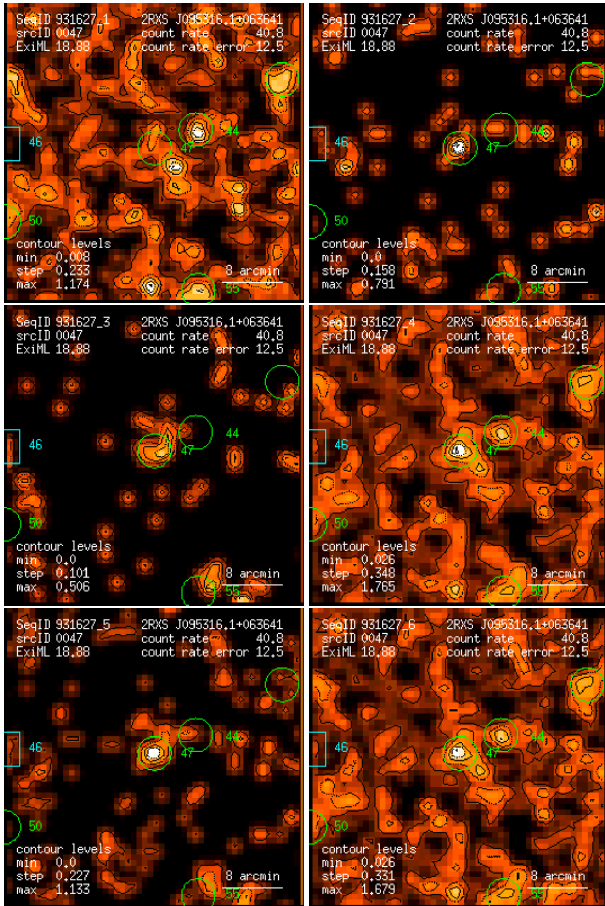
Figure 47: RASS 931627: detection 0047: band rate images, Gaussian filter: (1) PSPC channels 11 – 41, (2) 52 – 90, (3) 91 – 201, (4) 11 – 235, (5) 52 – 201, (6) 11 – 201. Broad band rates in counts/ks. Band rate contour levels in counts/ks/arcmin 2 .
