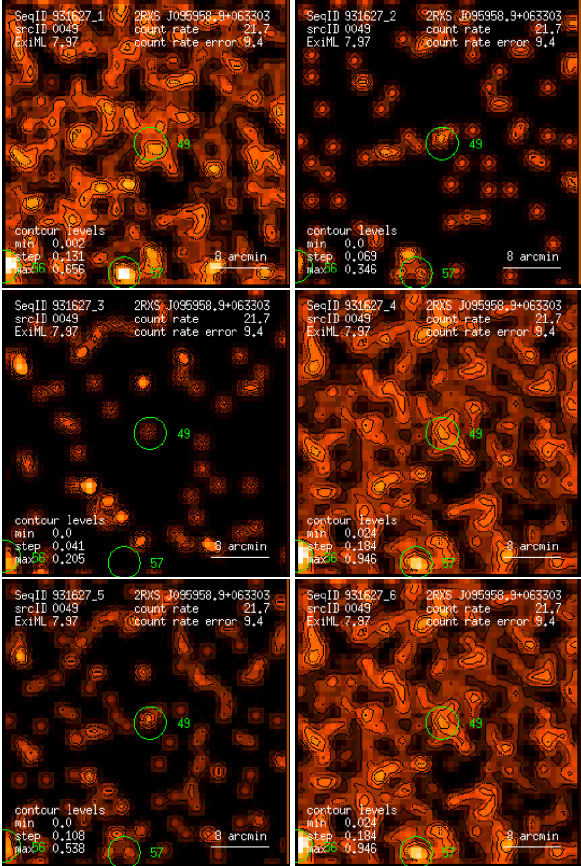
Figure 49: RASS 931627: detection 0049: band rate images, Gaussian filter: (1) PSPC channels 11 – 41, (2) 52 – 90, (3) 91 – 201, (4) 11 – 235, (5) 52 – 201, (6) 11 – 201. Broad band rates in counts/ks. Band rate contour levels in counts/ks/arcmin 2 .
