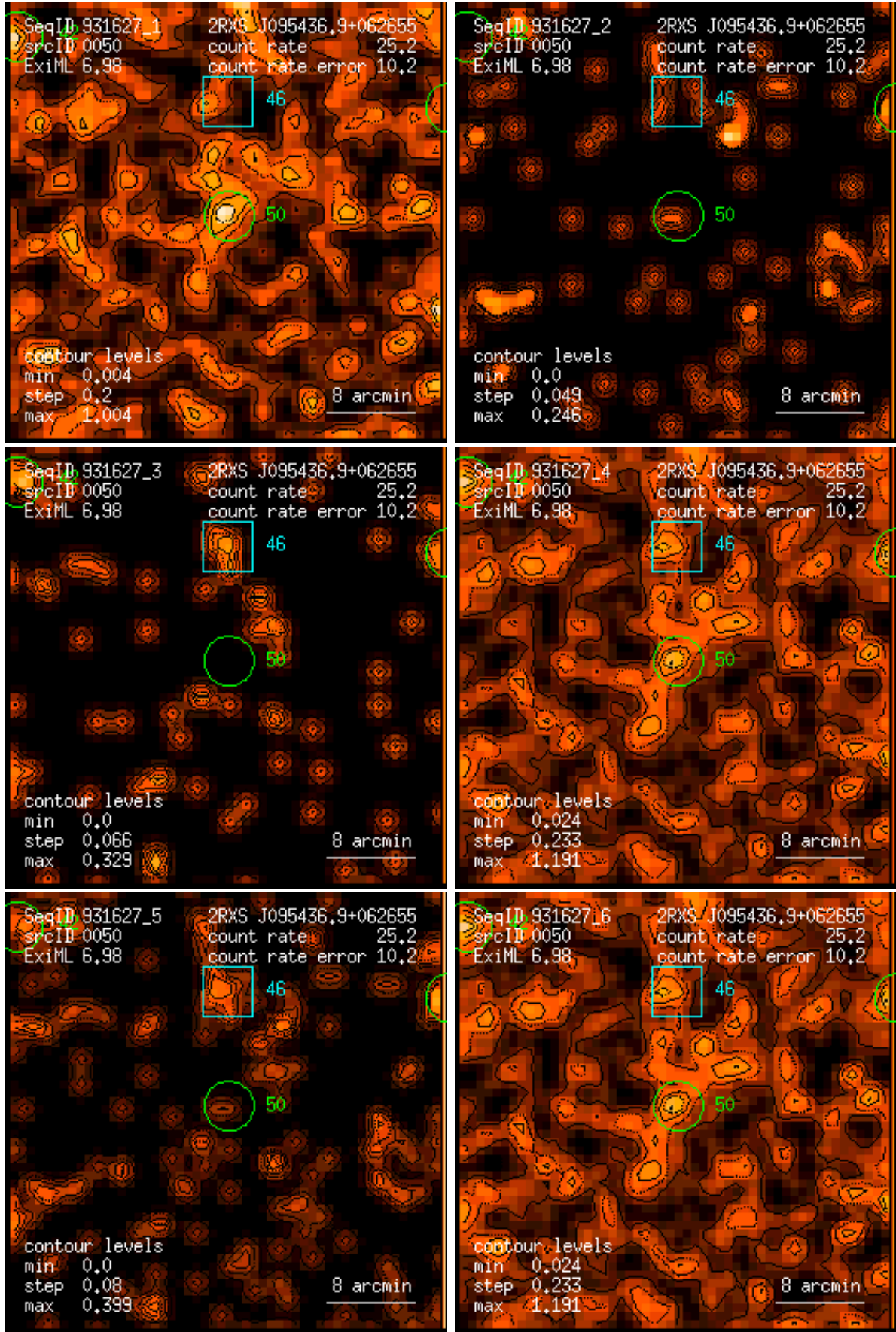
Figure 50: RASS 931627: detection 0050: band rate images, Gaussian filter: (1) PSPC channels 11 – 41, (2) 52 – 90, (3) 91 – 201, (4) 11 – 235, (5) 52 – 201, (6) 11 – 201. Broad band rates in counts/ks. Band rate contour levels in counts/ks/arcmin 2 .
