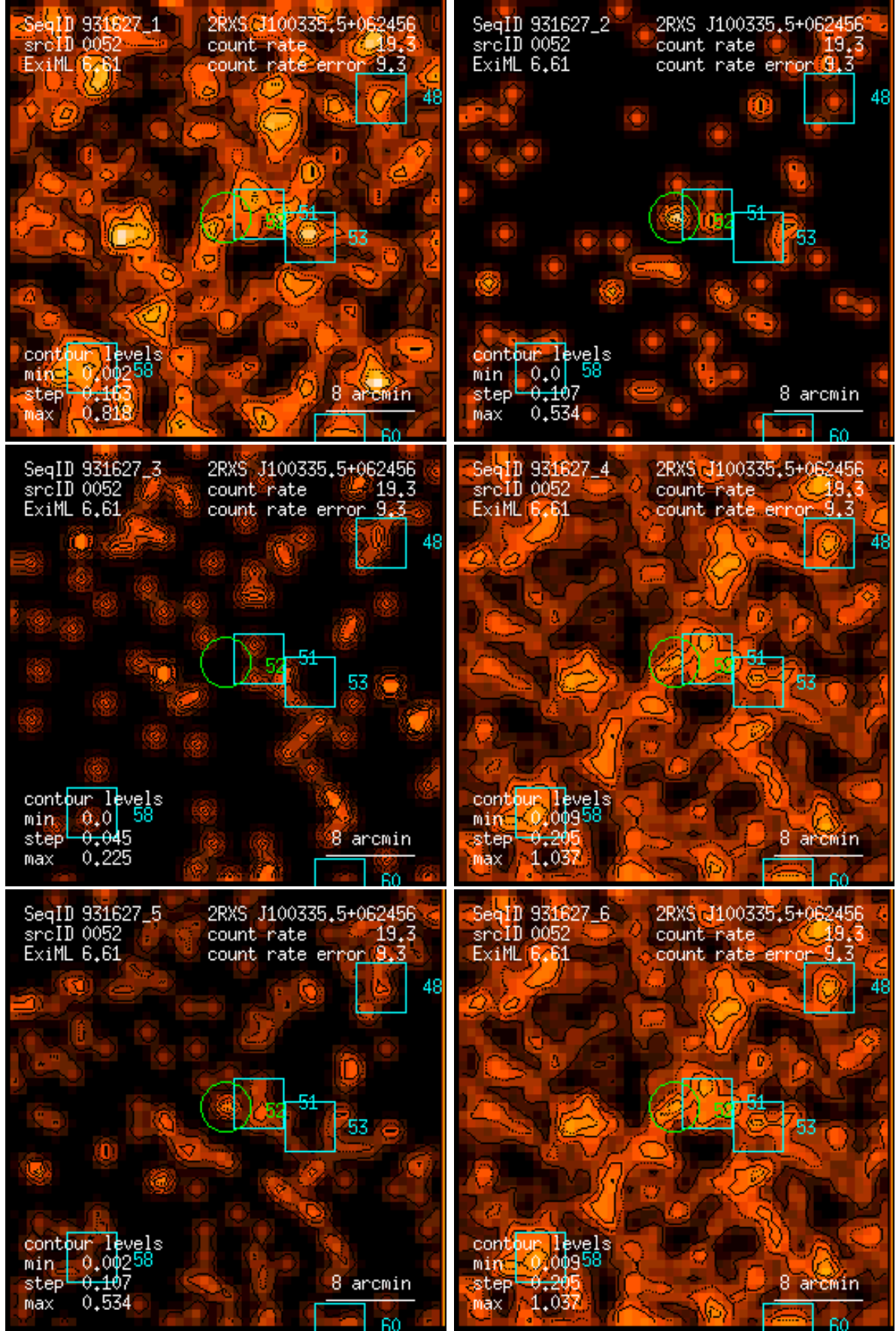
Figure 52: RASS 931627: detection 0052: band rate images, Gaussian filter: (1) PSPC channels 11 – 41, (2) 52 – 90, (3) 91 – 201, (4) 11 – 235, (5) 52 – 201, (6) 11 – 201. Broad band rates in counts/ks. Band rate contour levels in counts/ks/arcmin 2 .
