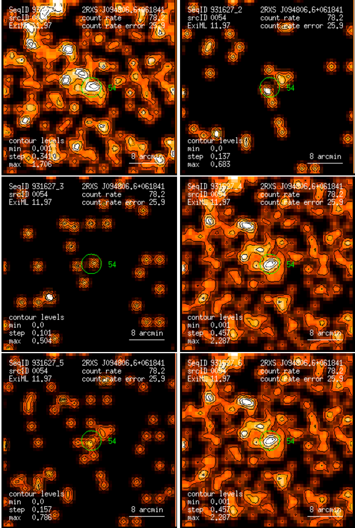
Figure 54: RASS 931627: detection 0054: band rate images, Gaussian filter: (1) PSPC channels 11 – 41, (2) 52 – 90, (3) 91 – 201, (4) 11 – 235, (5) 52 – 201, (6) 11 – 201. Broad band rates in counts/ks. Band rate contour levels in counts/ks/arcmin 2 .
