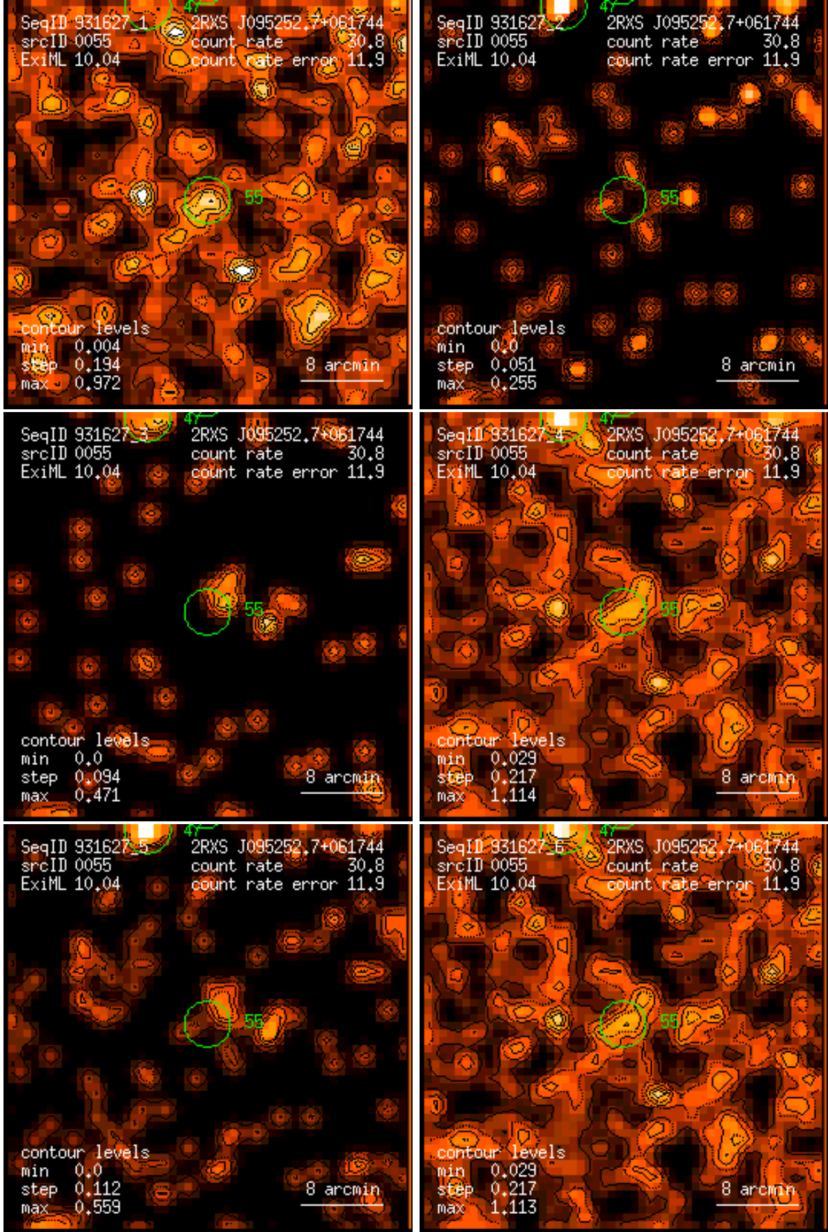
Figure 55: RASS 931627: detection 0055: band rate images, Gaussian filter: (1) PSPC channels 11 – 41, (2) 52 – 90, (3) 91 – 201, (4) 11 – 235, (5) 52 – 201, (6) 11 – 201. Broad band rates in counts/ks. Band rate contour levels in counts/ks/arcmin 2 .
