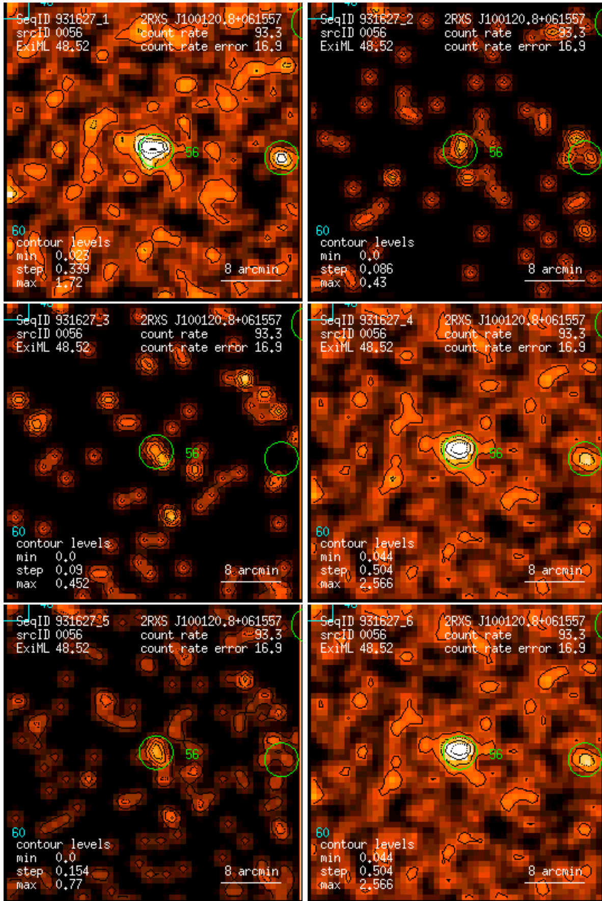
Figure 56: RASS 931627: detection 0056: band rate images, Gaussian filter: (1) PSPP channels 11 – 41, (2) 52 – 90, (3) 91 – 201, (4) 11 – 235, (5) 52 – 201, (6) 11 – 201. Broad band rates in counts/ks. Band rate contour levels in counts/ks/arcmin 2 .
