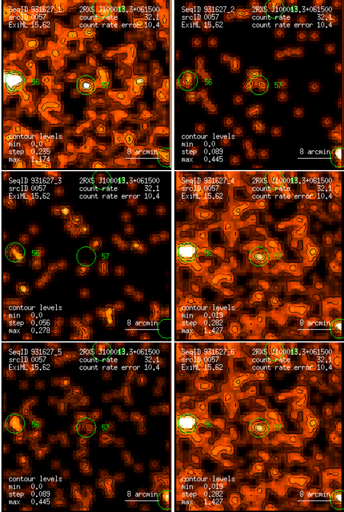
Figure 57: RASS 931627: detection 0057: band rate images, Gaussian filter: (1) PSPC channels 11 – 41, (2) 52 – 90, (3) 91 – 201, (4) 11 – 235, (5) 52 – 201, (6) 11 – 201. Broad band rates in counts/ks. Band rate contour levels in counts/ks/arcmin 2 .
