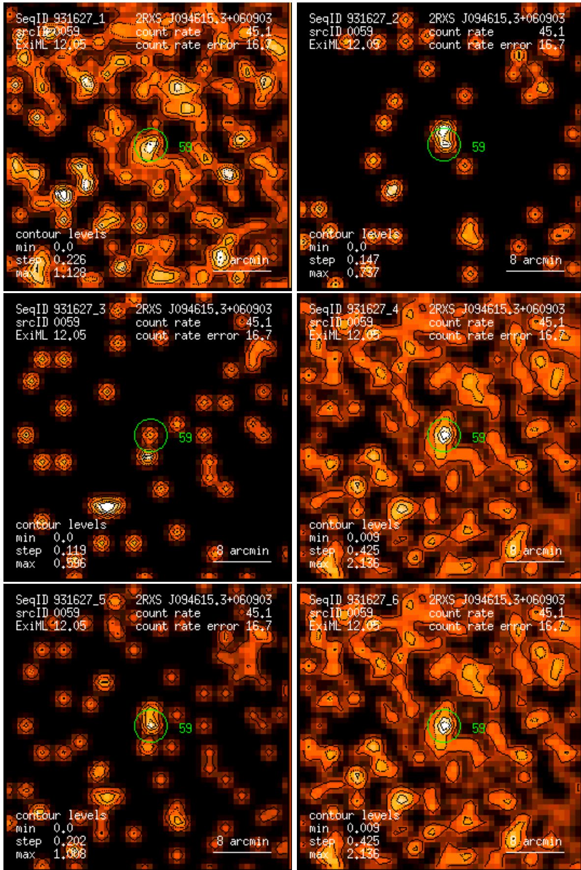
Figure 59: RASS 931627: detection 0059: band rate images, Gaussian filter: (1) PSPC channels 11 – 41, (2) 52 – 90, (3) 91 – 201, (4) 11 – 235, (5) 52 – 201, (6) 11 – 201. Broad band rates in counts/ks. Band rate contour levels in counts/ks/arcmin 2 .
