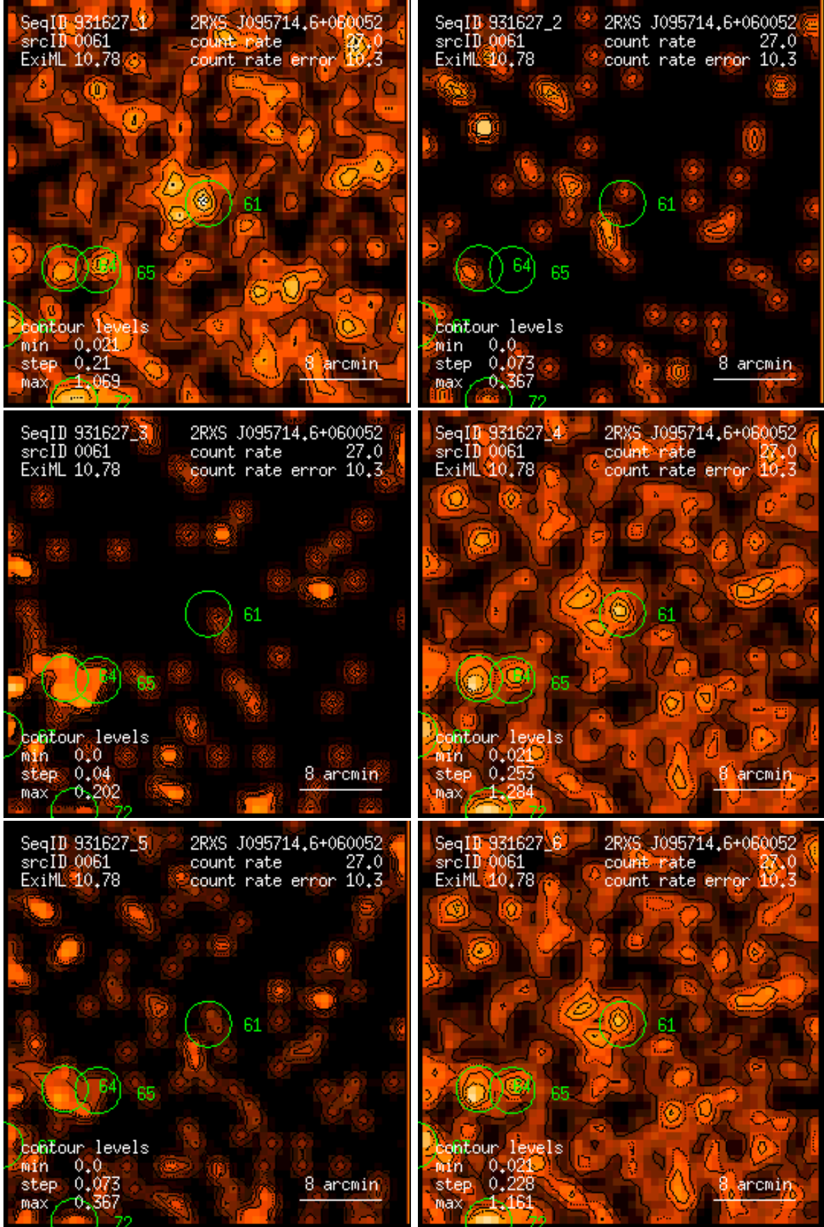
Figure 61: RASS 931627: detection 0061: band rate images, Gaussian filter: (1) PSPC channels 11 – 41, (2) 52 – 90, (3) 91 – 201, (4) 11 – 235, (5) 52 – 201, (6) 11 – 201. Broad band rates in counts/ks. Band rate contour levels in counts/ks/arcmin 2 .
