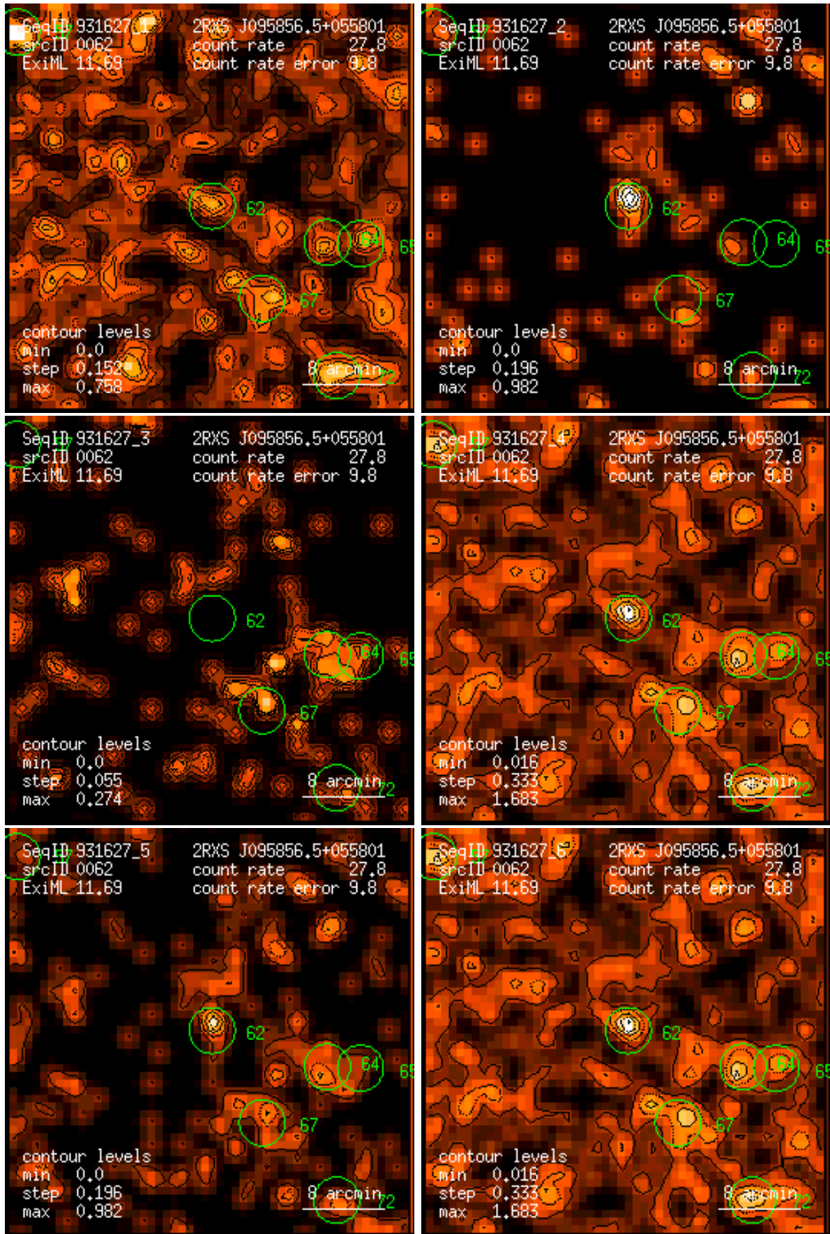
Figure 62: RASS 931627: detection 0062: band rate images, Gaussian filter: (1) PSPC channels 11 – 41, (2) 52 – 90, (3) 91 – 201, (4) 11 – 235, (5) 52 – 201, (6) 11 – 201. Broad band rates in counts/ks. Band rate contour levels in counts/ks/arcmin 2 .
