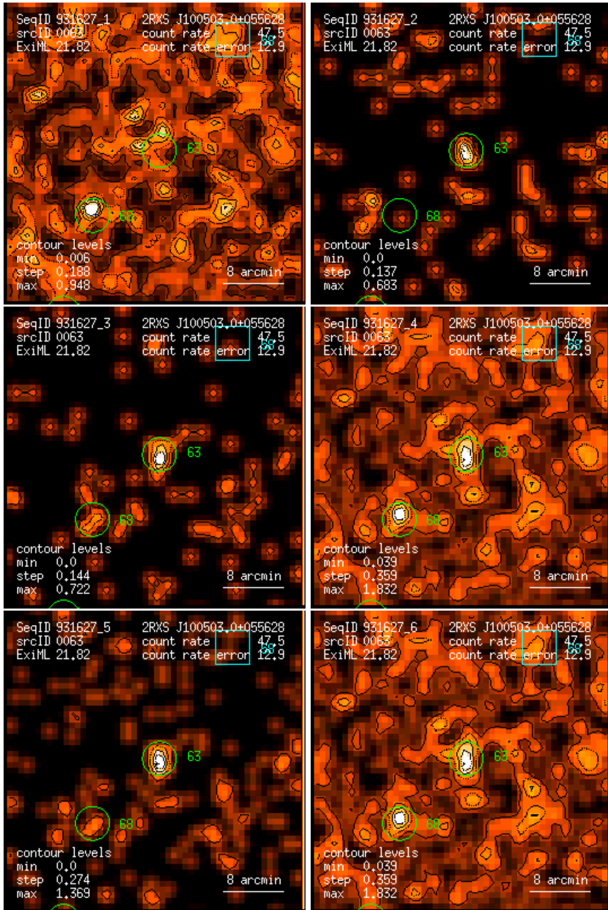
Figure 63: RASS 931627: detection 0063: band rate images, Gaussian filter: (1) PSPC channels 11 – 41, (2) 52 – 90, (3) 91 – 201, (4) 11 – 235, (5) 52 – 201, (6) 11 – 201. Broad band rates in counts/ks. Band rate contour levels in counts/ks/arcmin 2 .
