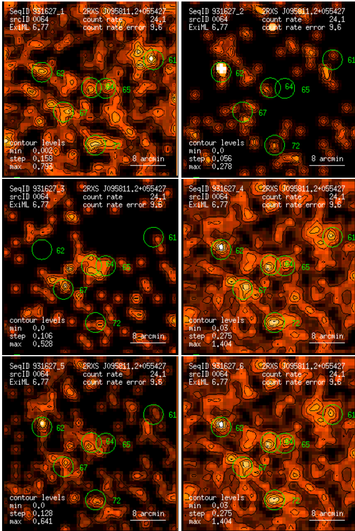
Figure 64: RASS 931627: detection 0064: band rate images, Gaussian filter: (1) PSPC channels 11 – 41, (2) 52 – 90, (3) 91 – 201, (4) 11 – 235, (5) 52 – 201, (6) 11 – 201. Broad band rates in counts/ks. Band rate contour levels in counts/ks/arcmin 2 .
