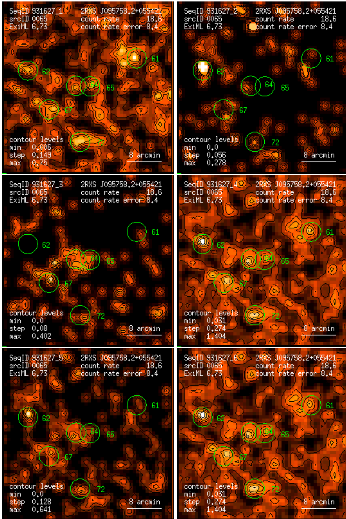
Figure 65: RASS 931627: detection 0065: band rate images, Gaussian filter: (1) PSPC channels 11 – 41, (2) 52 – 90, (3) 91 – 201, (4) 11 – 235, (5) 52 – 201, (6) 11 – 201. Broad band rates in counts/ks. Band rate contour levels in counts/ks/arcmin 2 .
