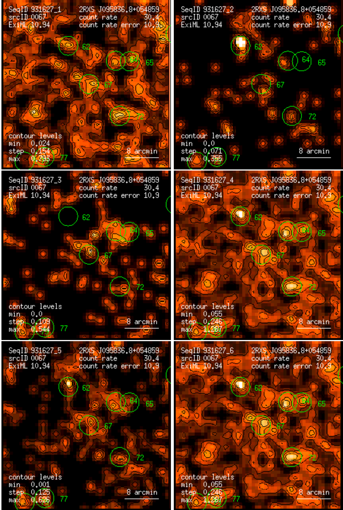
Figure 67: RASS 931627: detection 0067: band rate images, Gaussian filter: (1) PSPC channels 11 – 41, (2) 52 – 90, (3) 91 – 201, (4) 11 – 235, (5) 52 – 201, (6) 11 – 201. Broad band rates in counts/ks. Band rate contour levels in counts/ks/arcmin 2 .
