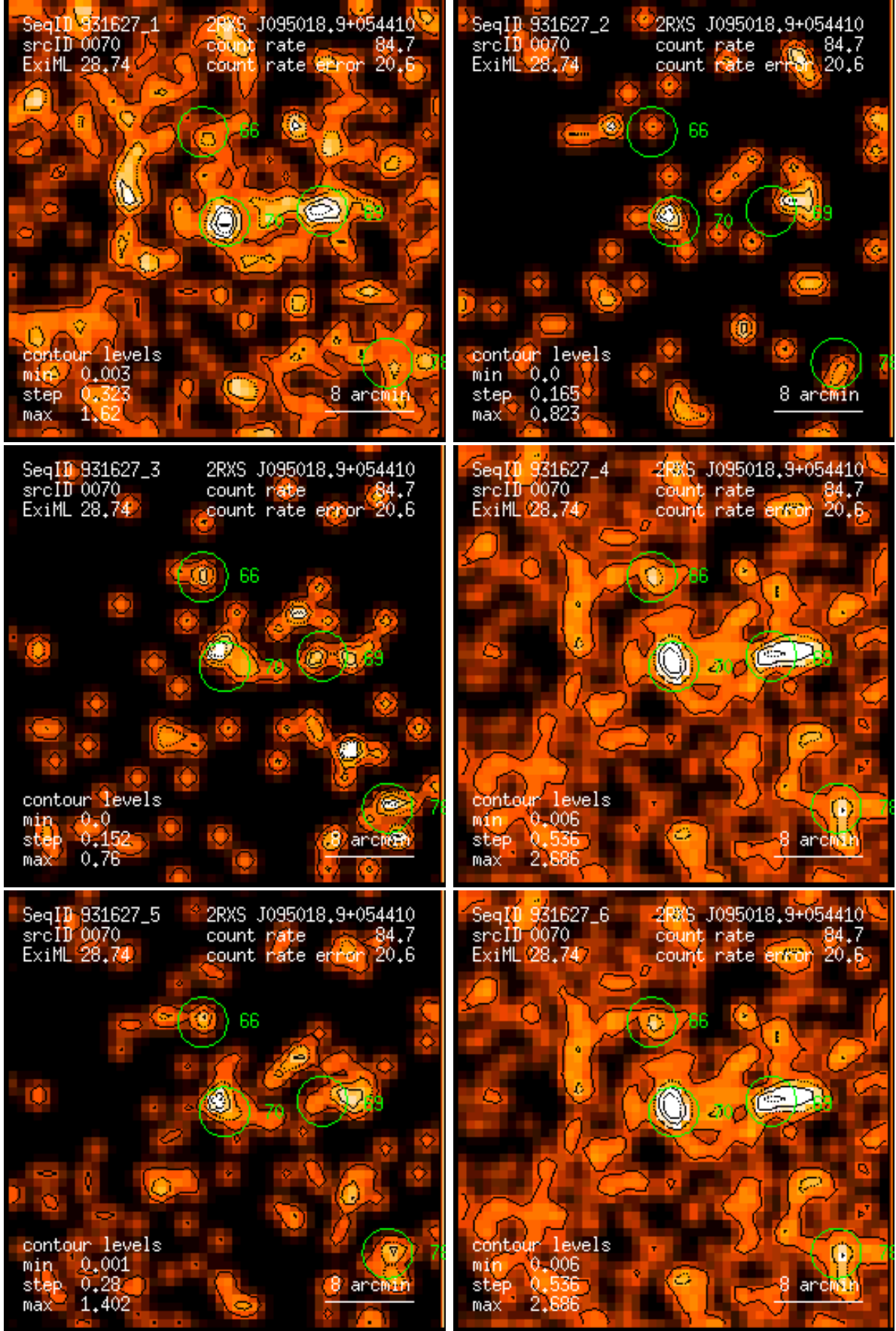
Figure 70: RASS 931627: detection 0070: band rate images, Gaussian filter: (1) PSPC channels 11 – 41, (2) 52 – 90, (3) 91 – 201, (4) 11 – 235, (5) 52 – 201, (6) 11 – 201. Broad band rates in counts/ks. Band rate contour levels in counts/ks/arcmin 2 .
