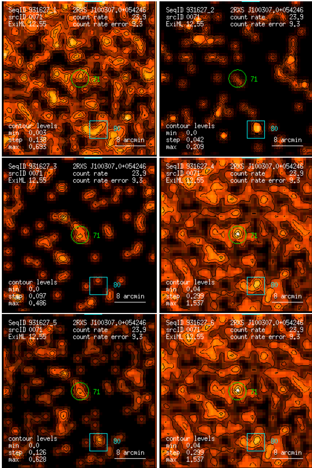
Figure 71: RASS 931627: detection 0071: band rate images, Gaussian filter: (1) PSPC channels 11 – 41, (2) 52 – 90, (3) 91 – 201, (4) 11 – 235, (5) 52 – 201, (6) 11 – 201. Broad band rates in counts/ks. Band rate contour levels in counts/ks/arcmin 2 .
