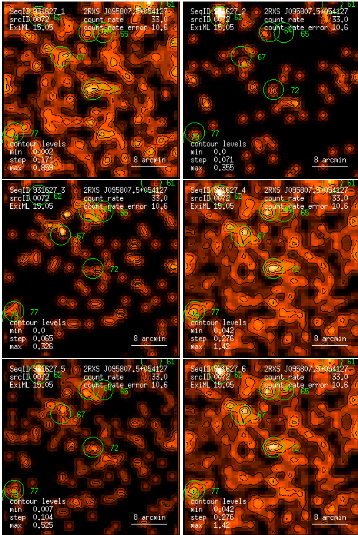
Figure 72: RASS 931627: detection 0072: band rate images, Gaussian filter: (1) PSPC channels 11 – 41, (2) 52 – 90, (3) 91 – 201, (4) 11 – 235, (5) 52 – 201, (6) 11 – 201. Broad band rates in counts/ks. Band rate contour levels in counts/ks/arcmin 2 .
