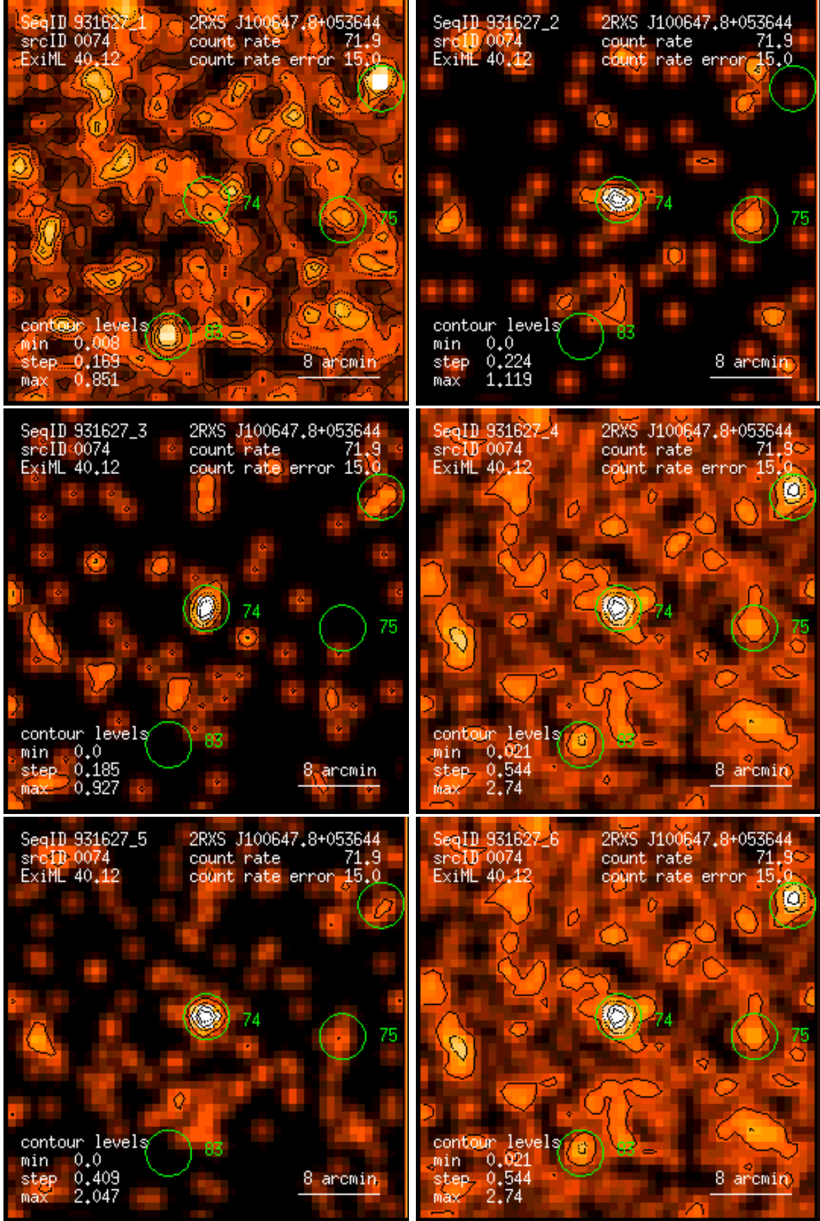
Figure 74: RASS 931627: detection 0074: band rate images, Gaussian filter: (1) PSPC channels 11 – 41, (2) 52 – 90, (3) 91 – 201, (4) 11 – 235, (5) 52 – 201, (6) 11 – 201. Broad band rates in counts/ks. Band rate contour levels in counts/ks/arcmin 2 .
