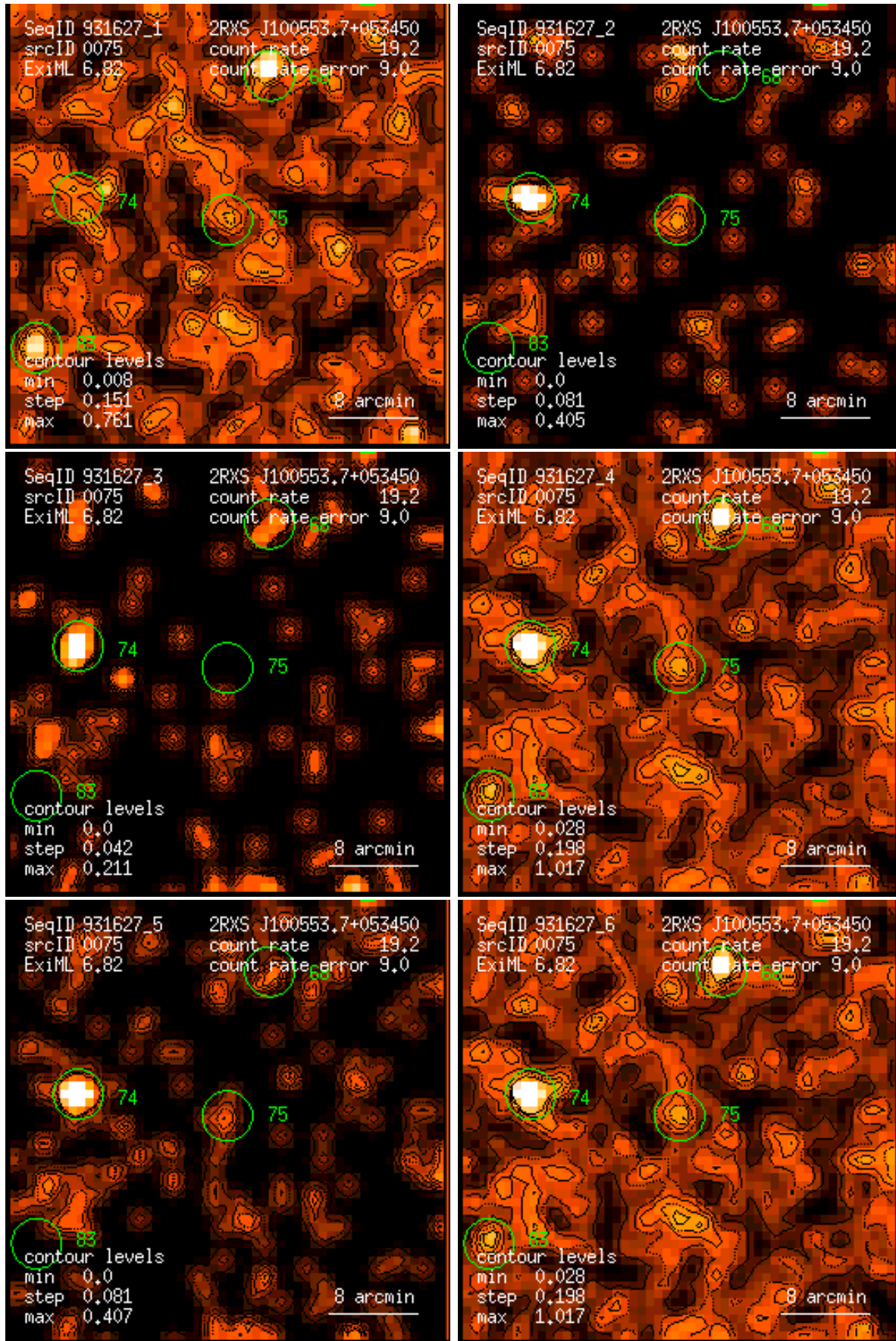
Figure 75: RASS 931627: detection 0075: band rate images, Gaussian filter: (1) PSPC channels 11 – 41, (2) 52 – 90, (3) 91 – 201, (4) 11 – 235, (5) 52 – 201, (6) 11 – 201. Broad band rates in counts/ks. Band rate contour levels in counts/ks/arcmin 2 .
