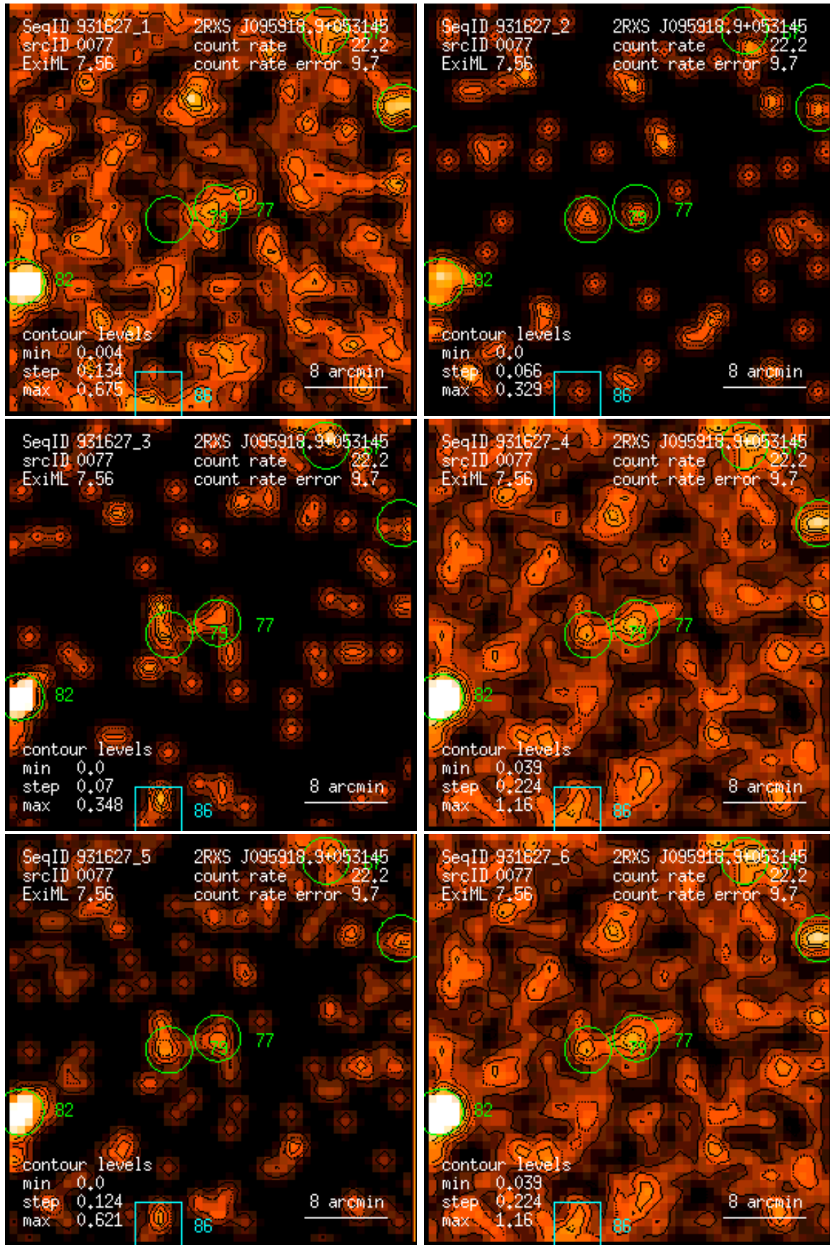
Figure 77: RASS 931627: detection 0077: band rate images, Gaussian filter: (1) PSPC channels 11 – 41, (2) 52 – 90, (3) 91 – 201, (4) 11 – 235, (5) 52 – 201, (6) 11 – 201. Broad band rates in counts/ks. Band rate contour levels in counts/ks/arcmin 2 .
