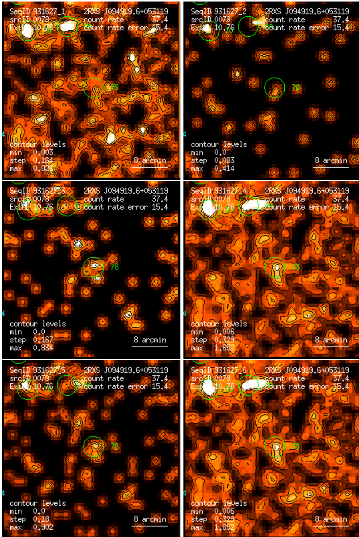
Figure 78: RASS 931627: detection 0078: band rate images, Gaussian filter: (1) PSPC channels 11 – 41, (2) 52 – 90, (3) 91 – 201, (4) 11 – 235, (5) 52 – 201, (6) 11 – 201. Broad band rates in counts/ks. Band rate contour levels in counts/ks/arcmin 2 .
