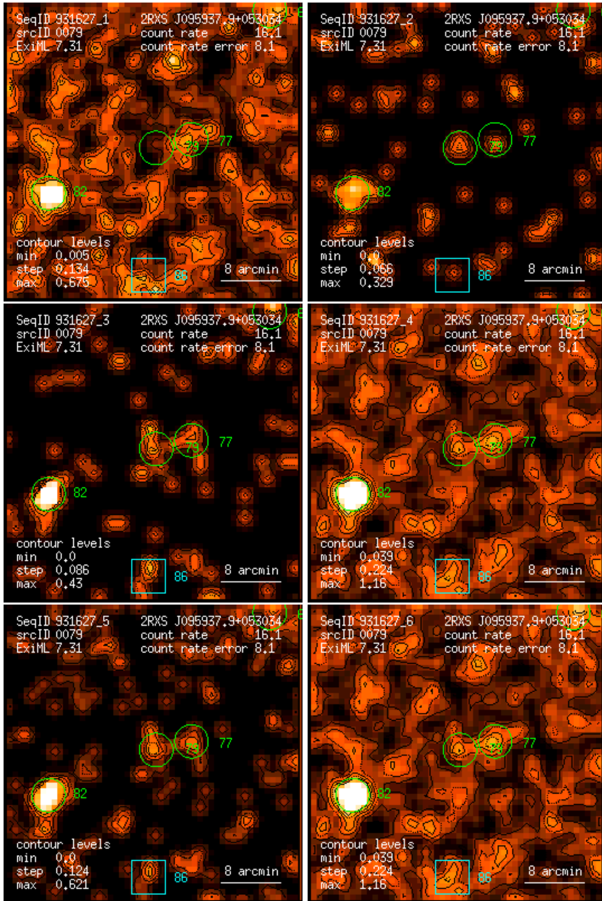
Figure 79: RASS 931627: detection 0079: band rate images, Gaussian filter: (1) PSPC channels 11 – 41, (2) 52 – 90, (3) 91 – 201, (4) 11 – 235, (5) 52 – 201, (6) 11 – 201. Broad band rates in counts/ks. Band rate contour levels in counts/ks/arcmin 2 .
