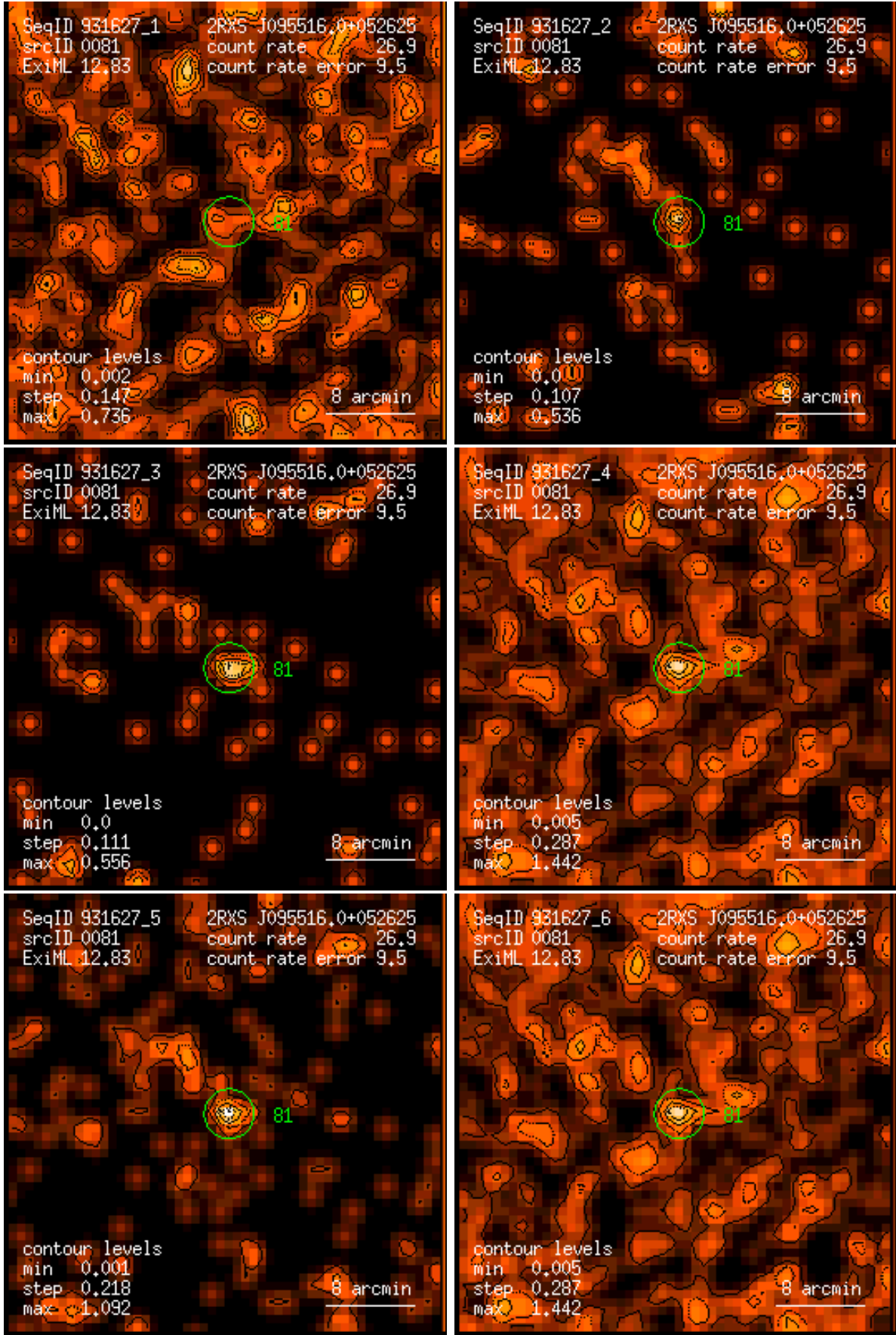
Figure 81: RASS 931627: detection 0081: band rate images, Gaussian filter: (1) PSPC channels 11 – 41, (2) 52 – 90, (3) 91 – 201, (4) 11 – 235, (5) 52 – 201, (6) 11 – 201. Broad band rates in counts/ks. Band rate contour levels in counts/ks/arcmin 2 .
