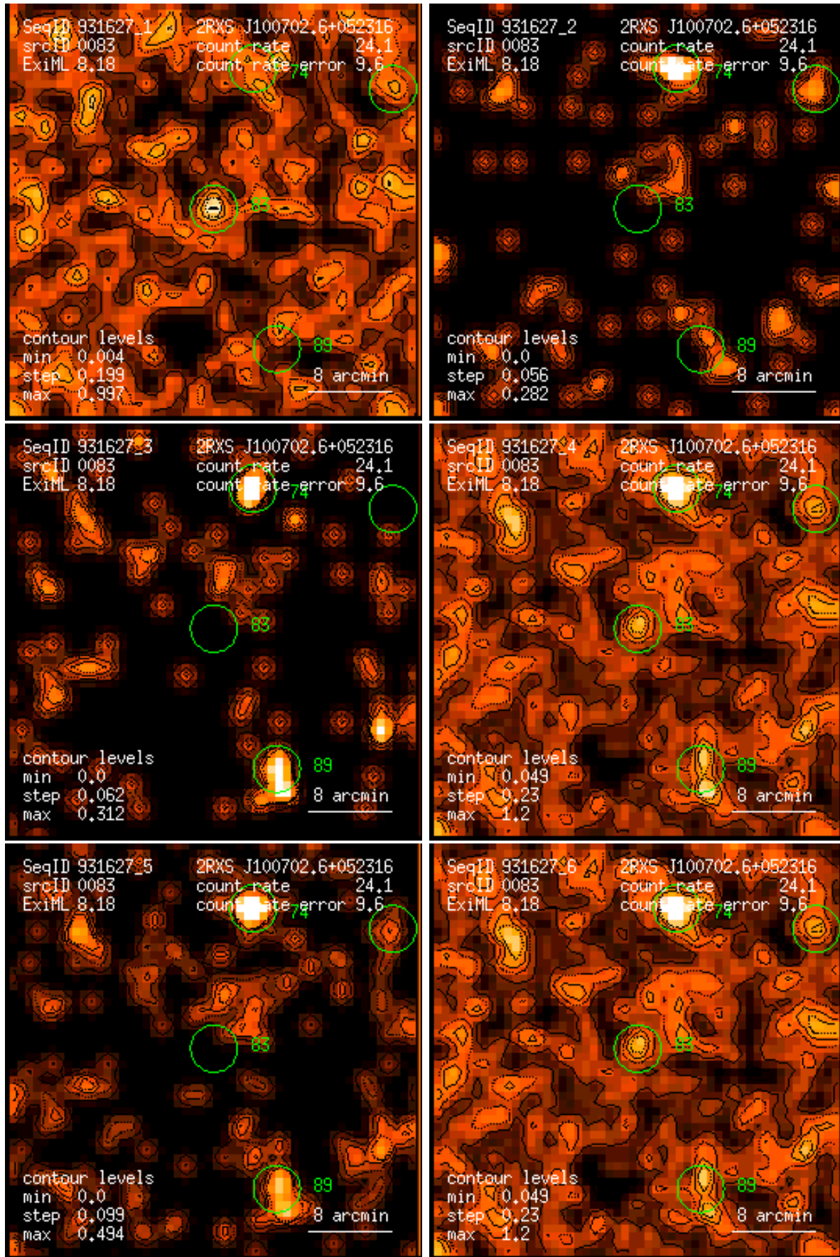
Figure 83: RASS 931627: detection 0083: band rate images, Gaussian filter: (1) PSPC channels 11 – 41, (2) 52 – 90, (3) 91 – 201, (4) 11 – 235, (5) 52 – 201, (6) 11 – 201. Broad band rates in counts/ks. Band rate contour levels in counts/ks/arcmin 2 .
