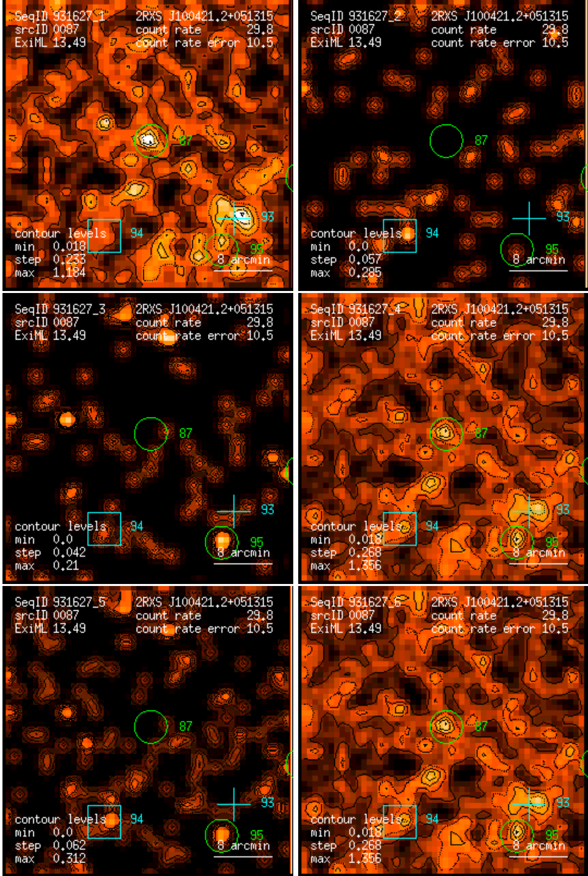
Figure 87: RASS 931627: detection 0087: band rate images, Gaussian filter: (1) PSPC channels 11 – 41, (2) 52 – 90, (3) 91 – 201, (4) 11 – 235, (5) 52 – 201, (6) 11 – 201. Broad band rates in counts/ks. Band rate contour levels in counts/ks/arcmin 2 .
