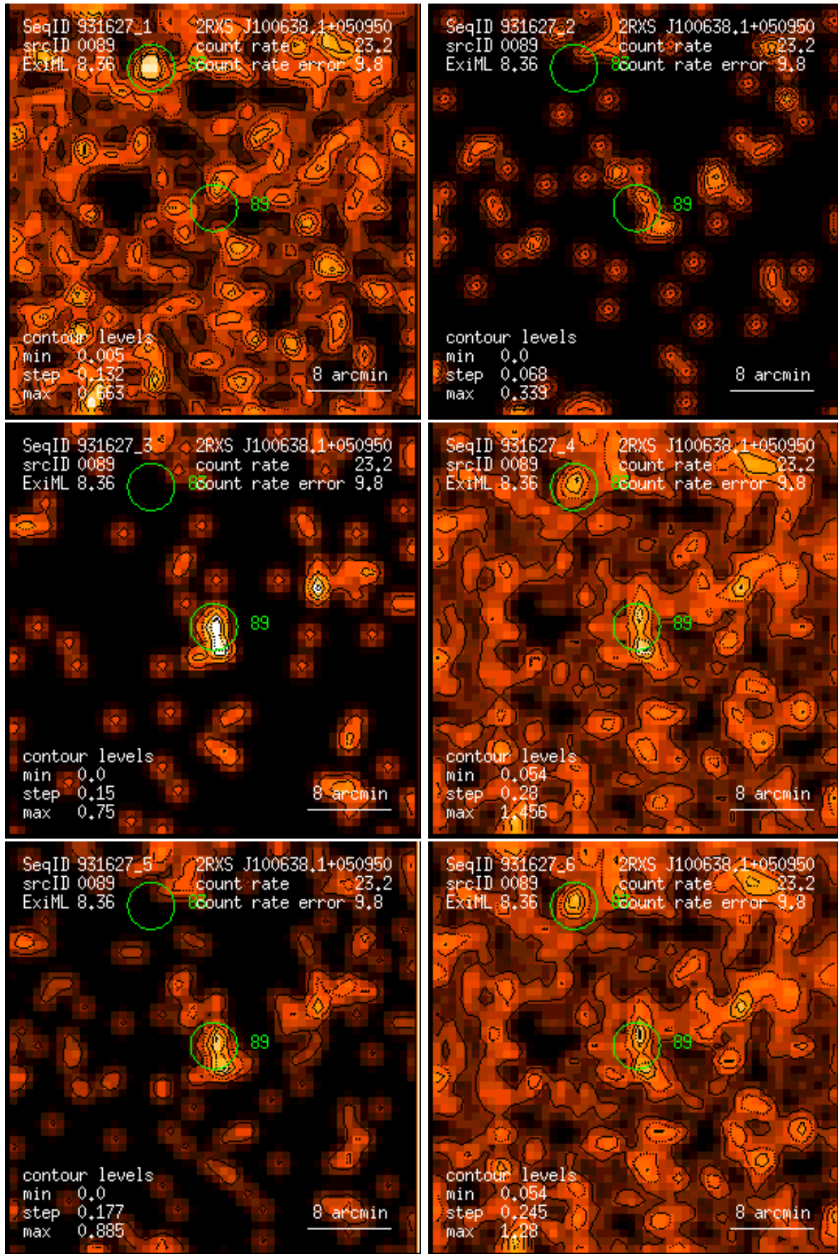
Figure 89: RASS 931627: detection 0089: band rate images, Gaussian filter: (1) PSPC channels 11 – 41, (2) 52 – 90, (3) 91 – 201, (4) 11 – 235, (5) 52 – 201, (6) 11 – 201. Broad band rates in counts/ks. Band rate contour levels in counts/ks/arcmin 2 .
