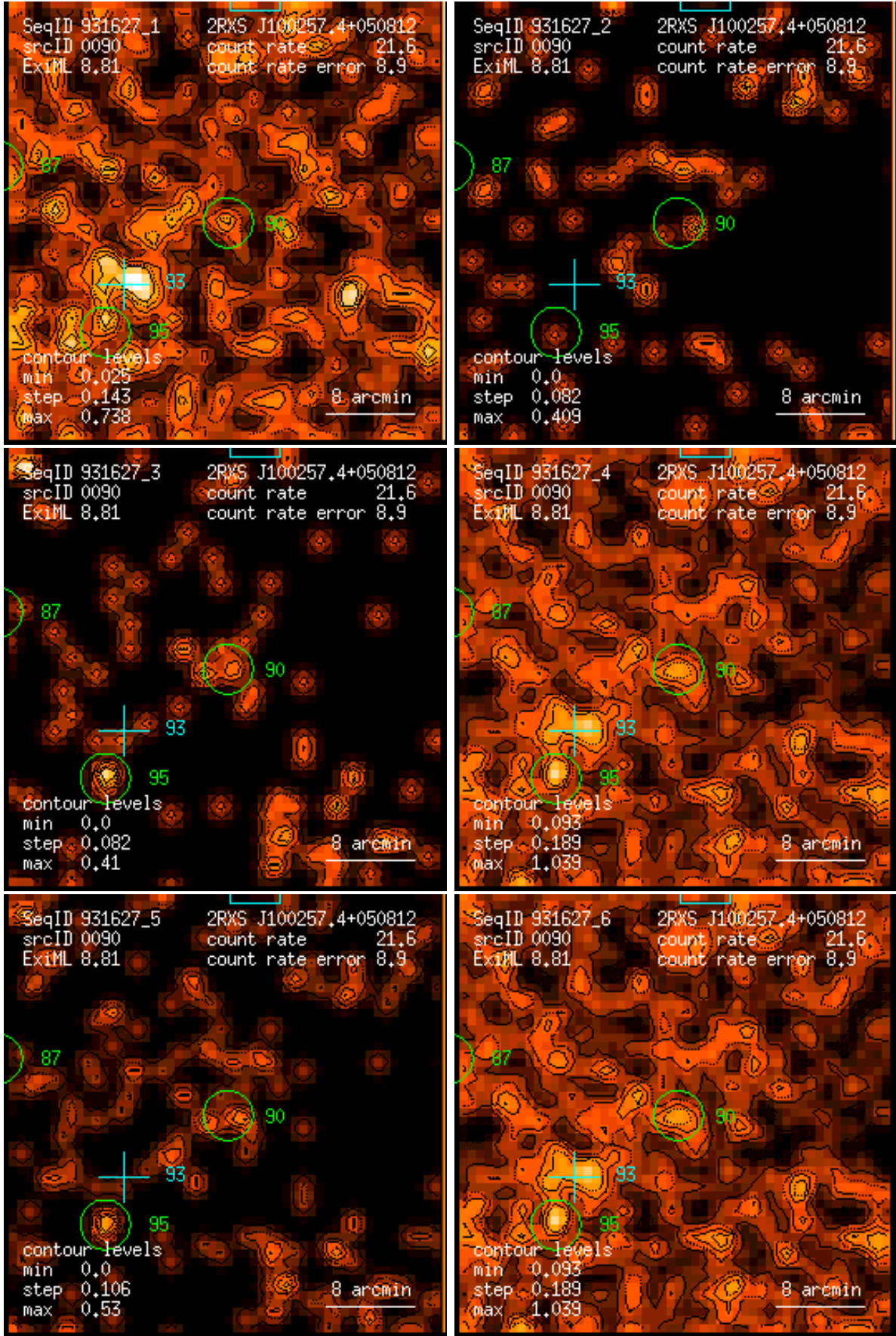
Figure 90: RASS 931627: detection 0090: band rate images, Gaussian filter: (1) PSPC channels 11 – 41, (2) 52 – 90, (3) 91 – 201, (4) 11 – 235, (5) 52 – 201, (6) 11 – 201. Broad band rates in counts/ks. Band rate contour levels in counts/ks/arcmin 2 .
