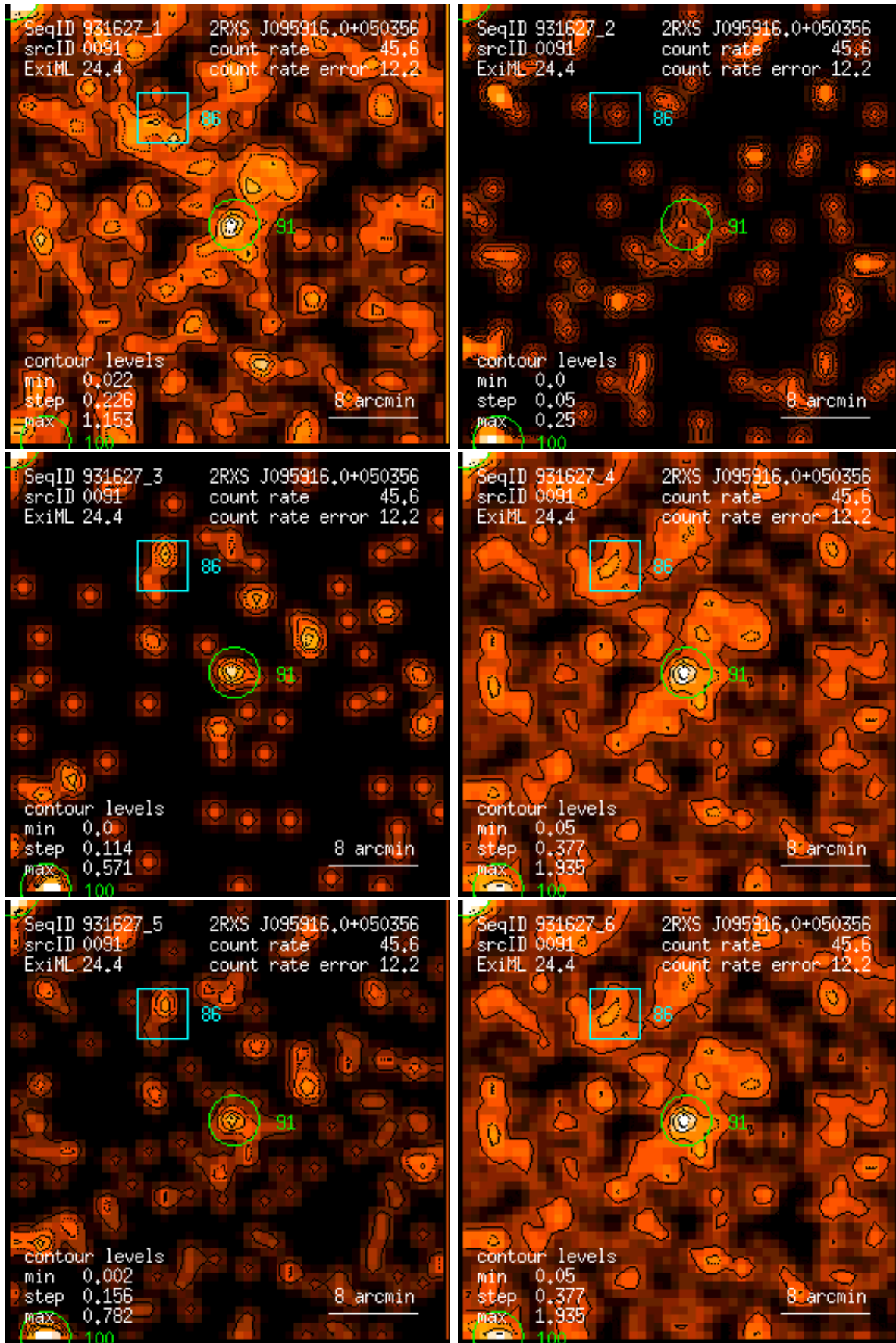
Figure 91: RASS 931627: detection 0091: band rate images, Gaussian filter: (1) PSPC channels 11 – 41, (2) 52 – 90, (3) 91 – 201, (4) 11 – 235, (5) 52 – 201, (6) 11 – 201. Broad band rates in counts/ks. Band rate contour levels in counts/ks/arcmin 2 .
