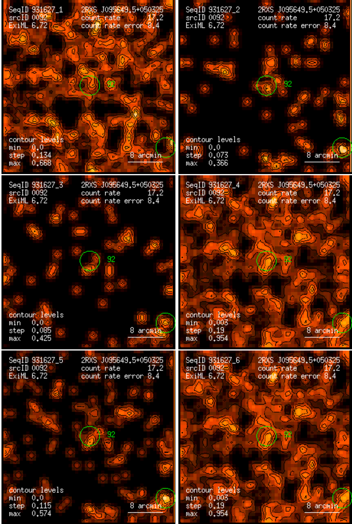
Figure 92: RASS 931627: detection 0092: band rate images, Gaussian filter: (1) PSPC channels 11 – 41, (2) 52 – 90, (3) 91 – 201, (4) 11 – 235, (5) 52 – 201, (6) 11 – 201. Broad band rates in counts/ks. Band rate contour levels in counts/ks/arcmin 2 .
