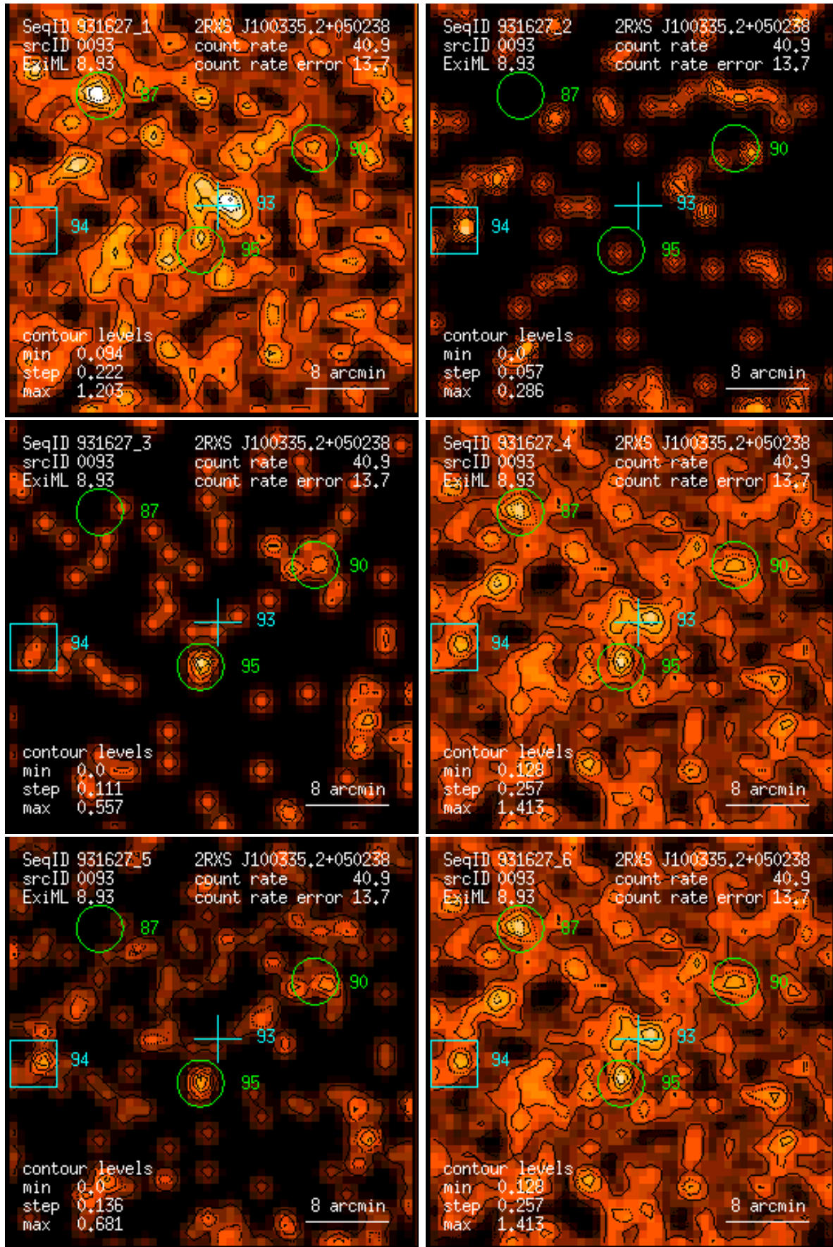
Figure 93: RASS 931627: detection 0093: band rate images, Gaussian filter: (1) PSPC channels 11 – 41, (2) 52 – 90, (3) 91 – 201, (4) 11 – 235, (5) 52 – 201, (6) 11 – 201. Broad band rates in counts/ks. Band rate contour levels in counts/ks/arcmin 2 .
