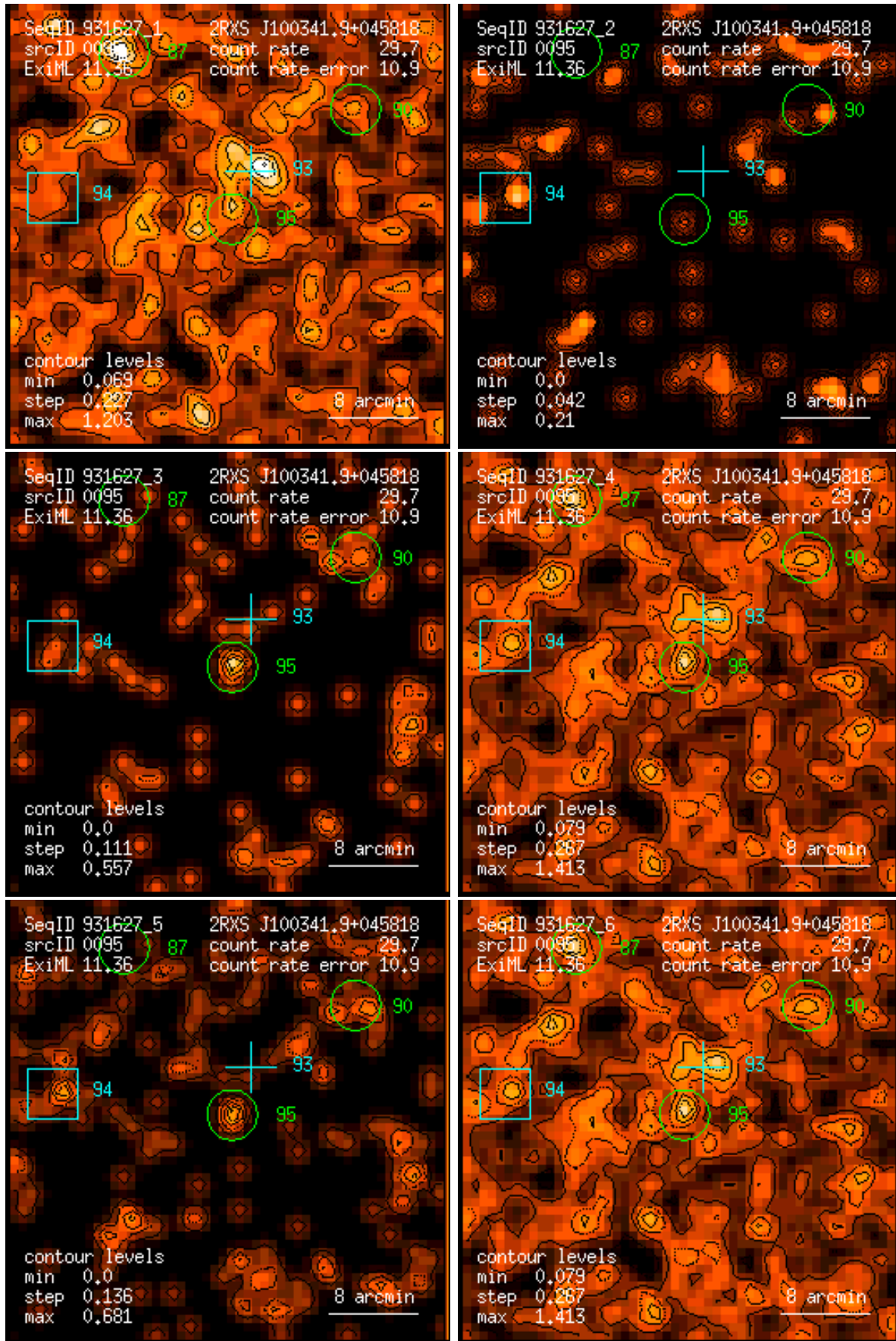
Figure 95: RASS 931627: detection 0095: band rate images, Gaussian filter: (1) PSPC channels 11 – 41, (2) 52 – 90, (3) 91 – 201, (4) 11 – 235, (5) 52 – 201, (6) 11 – 201. Broad band rates in counts/ks. Band rate contour levels in counts/ks/arcmin 2 .
