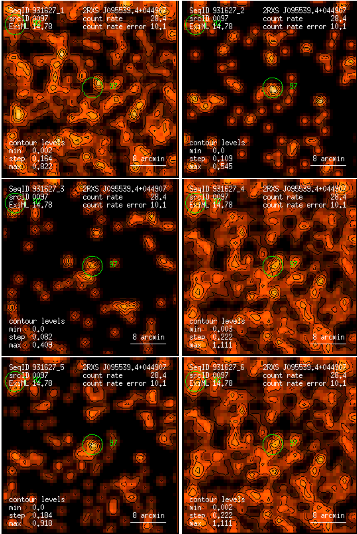
Figure 97: RASS 931627: detection 0097: band rate images, Gaussian filter: (1) PSPC channels 11 – 41, (2) 52 – 90, (3) 91 – 201, (4) 11 – 235, (5) 52 – 201, (6) 11 – 201. Broad band rates in counts/ks. Band rate contour levels in counts/ks/arcmin 2 .
