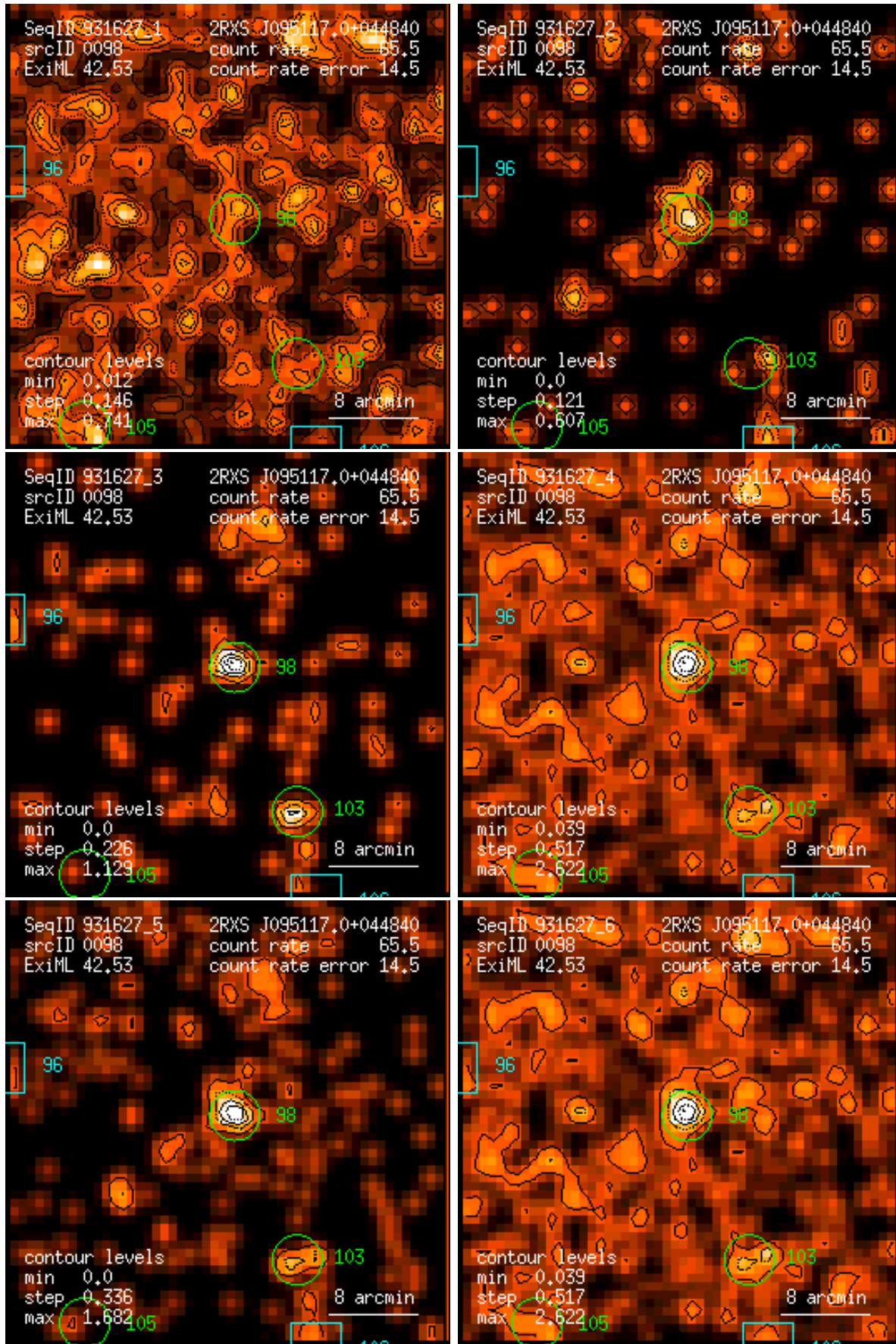
Figure 98: RASS 931627: detection 0098: band rate images, Gaussian filter: (1) PSPC channels 11 – 41, (2) 52 – 90, (3) 91 – 201, (4) 11 – 235, (5) 52 – 201, (6) 11 – 201. Broad band rates in counts/ks. Band rate contour levels in counts/ks/arcmin 2 .
