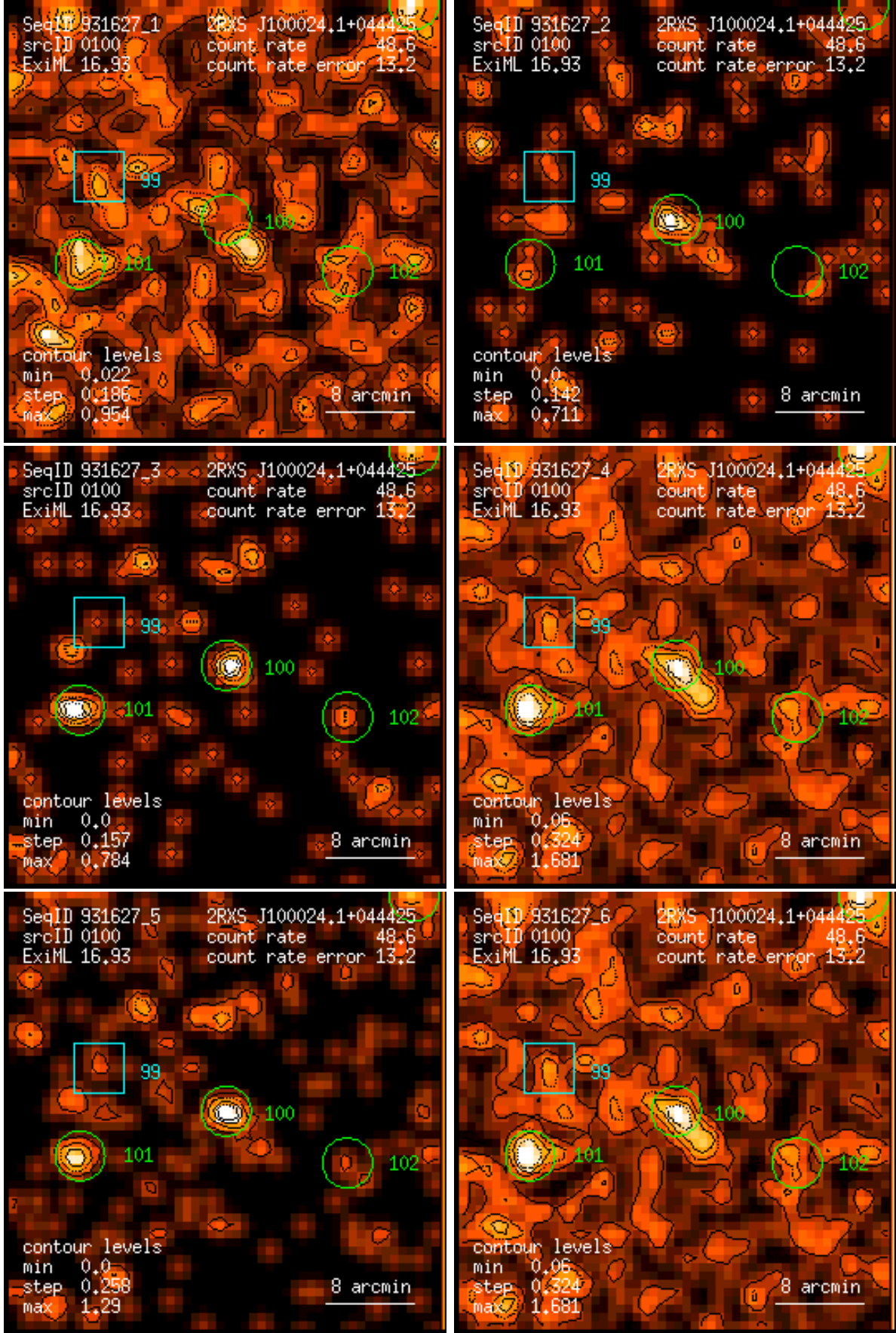
Figure 100: RASS 931627: detection 0100: band rate images, Gaussian filter: (1) PSPC channels 11 – 41, (2) 52 – 90, (3) 91 – 201, (4) 11 – 235, (5) 52 – 201, (6) 11 – 201. Broad band rates in counts/ks. Band rate contour levels in counts/ks/arcmin 2 .
