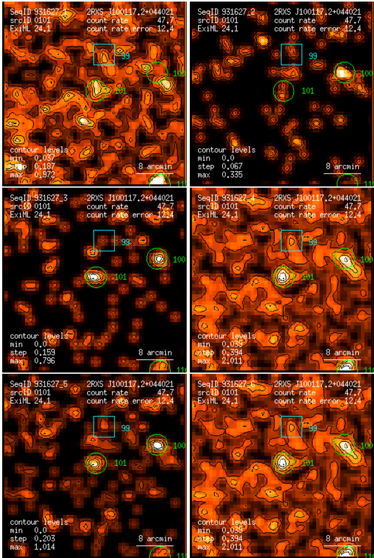
Figure 101: RASS 931627: detection 0101: band rate images, Gaussian filter: (1) PSPC channels 11 – 41, (2) 52 – 90, (3) 91 – 201, (4) 11 – 235, (5) 52 – 201, (6) 11 – 201. Broad band rates in counts/ks. Band rate contour levels in counts/ks/arcmin 2 .
