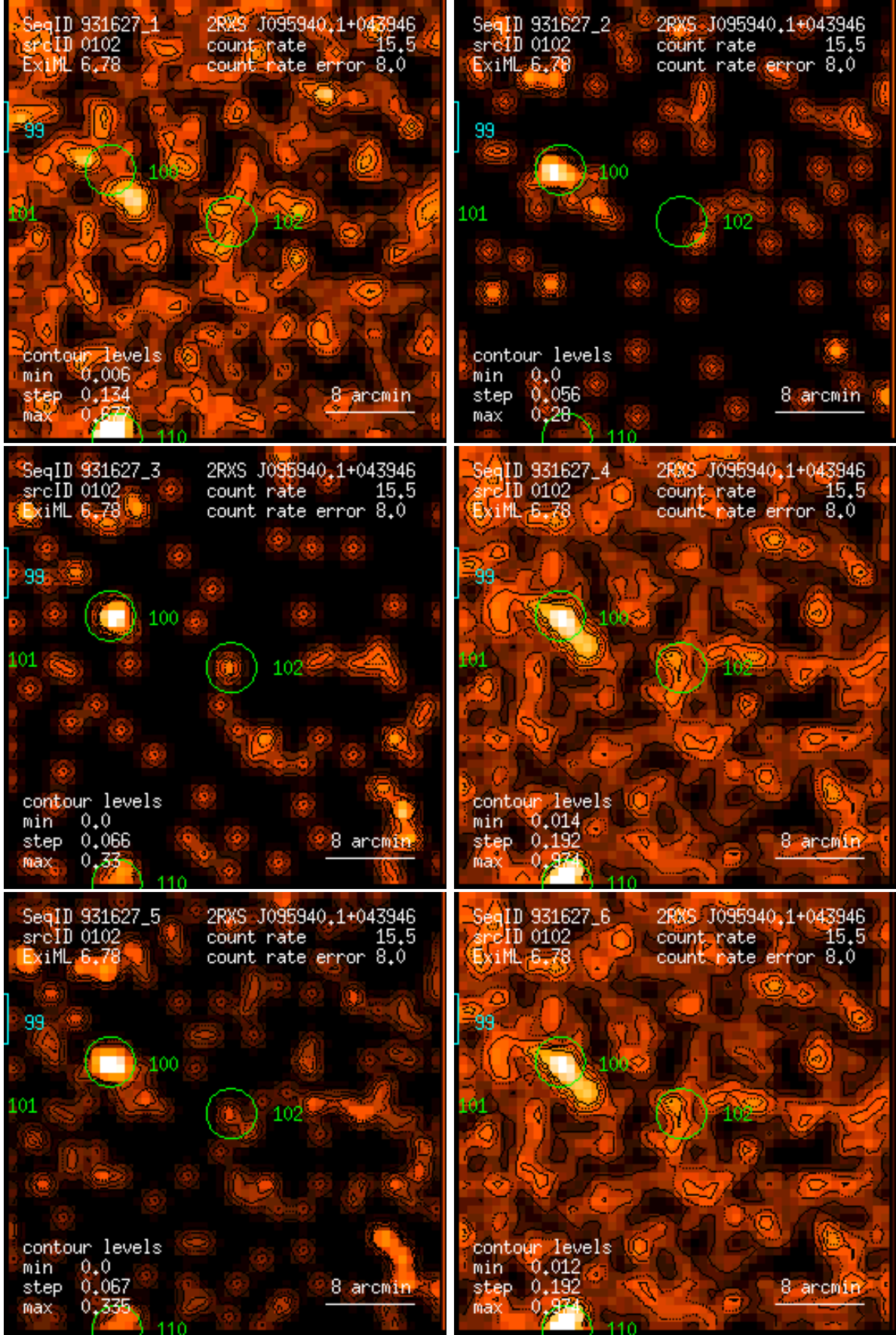
Figure 102: RASS 931627: detection 0102: band rate images, Gaussian filter: (1) PSPC channels 11 – 41, (2) 52 – 90, (3) 91 – 201, (4) 11 – 235, (5) 52 – 201, (6) 11 – 201. Broad band rates in counts/ks. Band rate contour levels in counts/ks/arcmin 2 .
