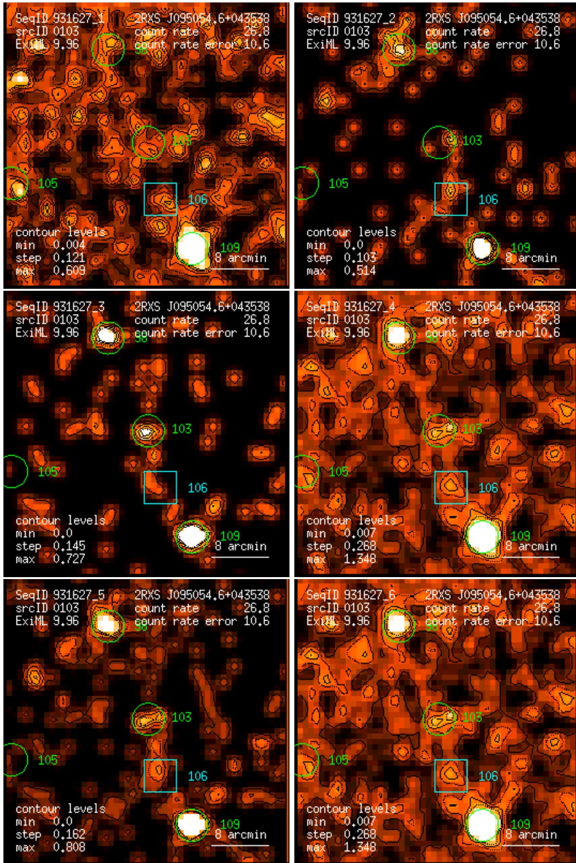
Figure 103: RASS 931627: detection 0103: band rate images, Gaussian filter: (1) PSPC channels 11 – 41, (2) 52 – 90, (3) 91 – 201, (4) 11 – 235, (5) 52 – 201, (6) 11 – 201. Broad band rates in counts/ks. Band rate contour levels in counts/ks/arcmin 2 .
