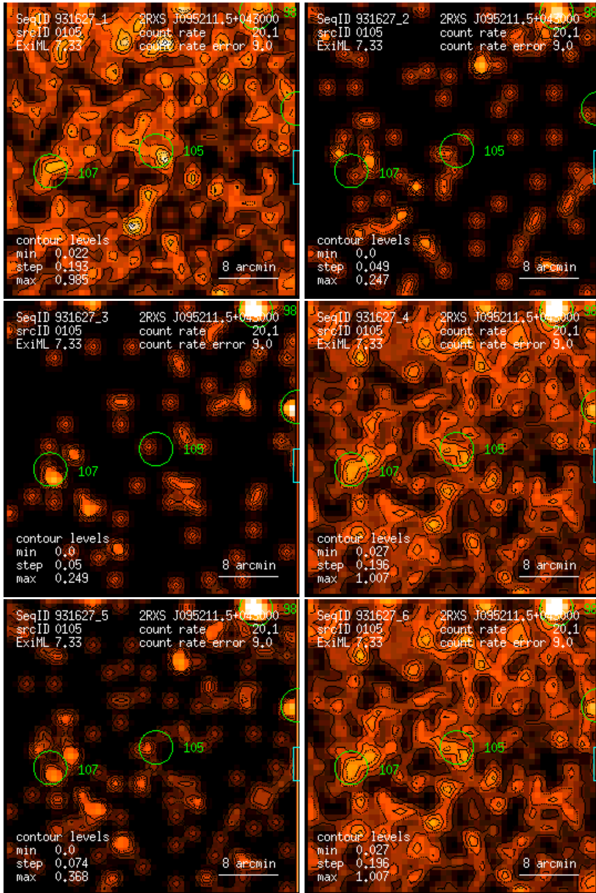
Figure 105: RASS 931627: detection 0105: band rate images, Gaussian filter: (1) PSPC channels 11 – 41, (2) 52 – 90, (3) 91 – 201, (4) 11 – 235, (5) 52 – 201, (6) 11 – 201. Broad band rates in counts/ks. Band rate contour levels in counts/ks/arcmin 2 .
